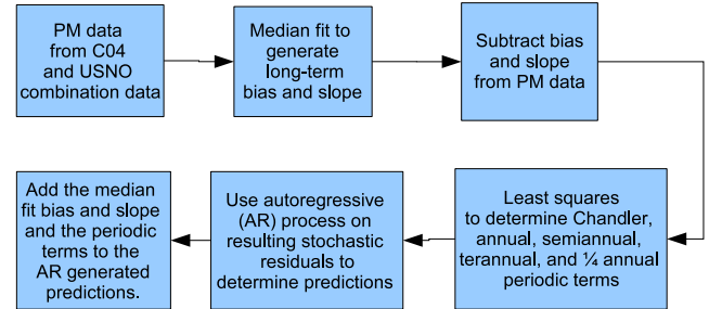
Figure 2: Polar Motion Least Squares / Auto Regression (LS/AR) Polar Motion Prediction Algorithm
