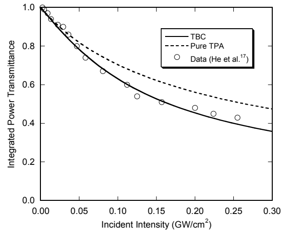
Figure 6. Nonlinear transmittance vs. incident intensity. Pure TPA, \beta = 9.46 cm/GW (dashed); \beta = 9.46 cm/GW, g = 1800 cm 3 /GW 2 , \gamma_{\text{eff}} = 120 cm 2 /GW 2 , \eta = 0.04 (solid). Circles are data according to He et al. 17
