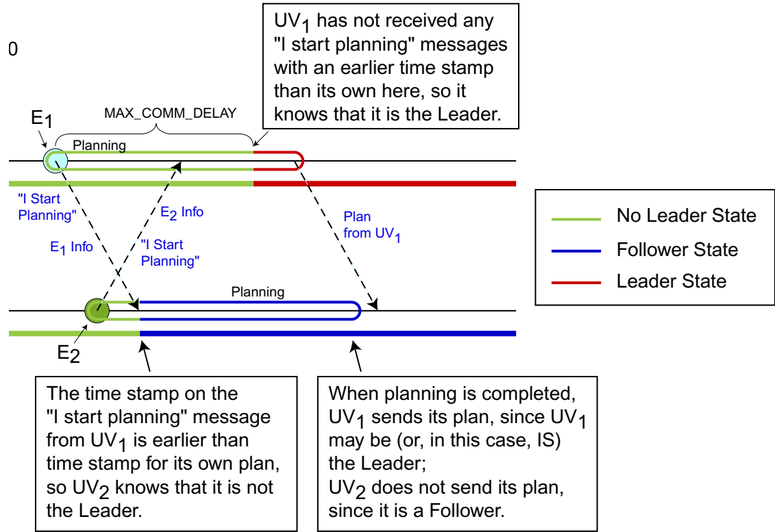
Figure 1. This figure shows the basic structure of the message transfer and leader state transitions of the DCGO protocol. Both vehicles start out as potential leaders, but after coordination, UV1 becomes the leader because it can react to information the fastest.
