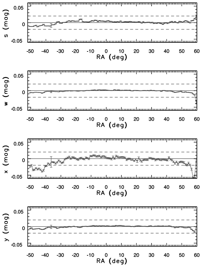
FIG. 10.—Dependence of the position of the stellar locus in ugriz color space, as parameterized by the median principal colors s_{\text{med}} , as a function of right ascension. Close to the edges, the median colors deviate significantly from zero. This is caused by intrinsic changes in the stellar locus due to stellar population variations and overestimated interstellar extinction corrections for red stars, rather than calibration problems. [See the electronic edition of the Journal for a color version of this figure.]
