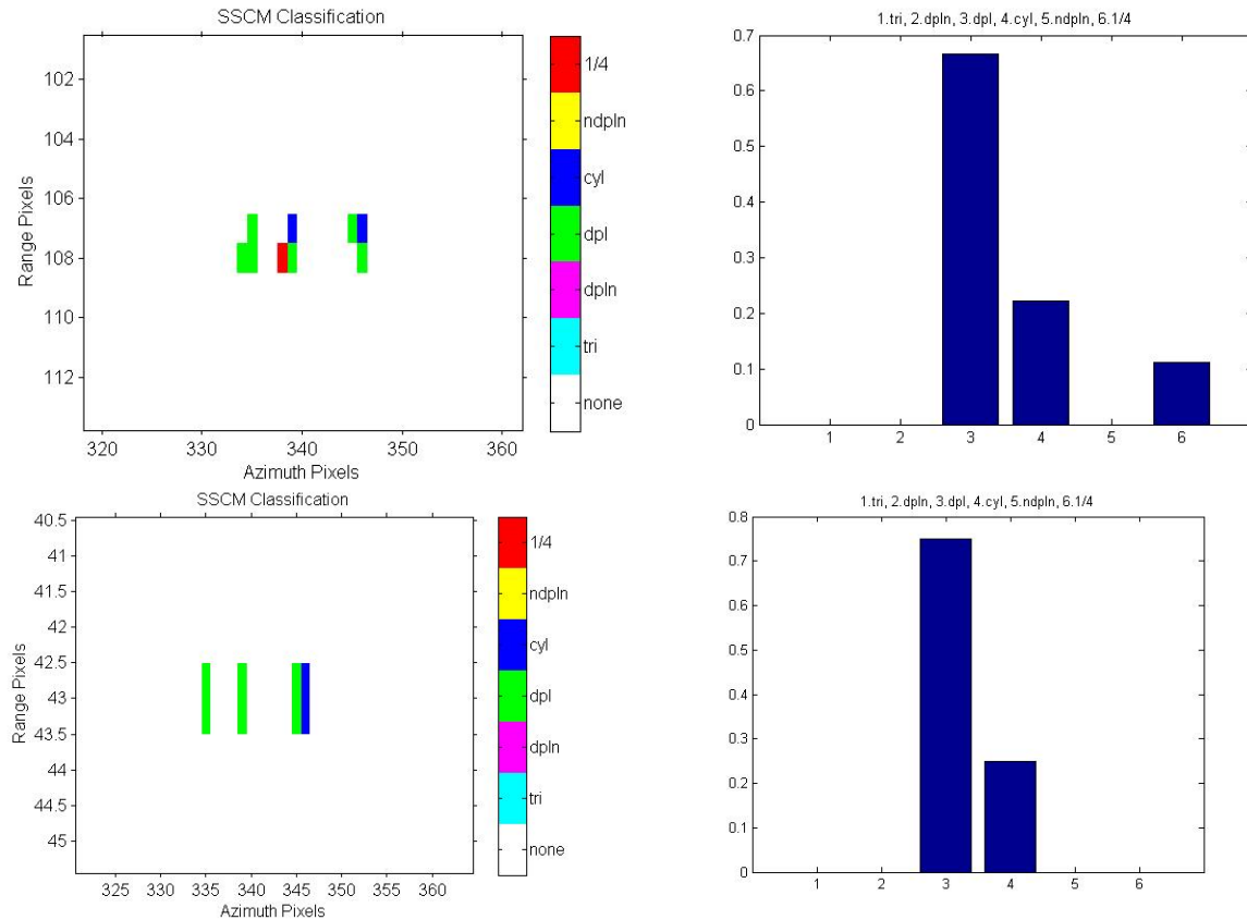
Figure 16: SSCM classification image (left) and histogram (right) of Dominion Victory (l41p1, 20 October 2005). Top: Fine Quad-Pol Mode; bottom: Standard Quad-Pol Mode. In the histograms (right): the scatterer type is along the x-axis and the percentage of the distribution is along the y-axis.
