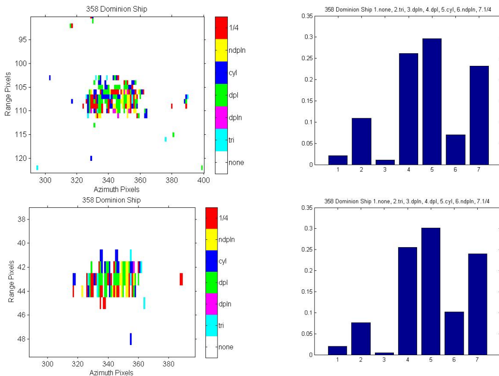
Figure 14: Cameron decomposition image (left) and histogram (right) of Dominion Victory (l41p1 20 October 2005). Top: Fine Quad-Pol, Bottom: Standard Quad-Pol. In the histograms (right): the scatterer type is along the x-axis and the percentage of the distribution is along the y-axis.
