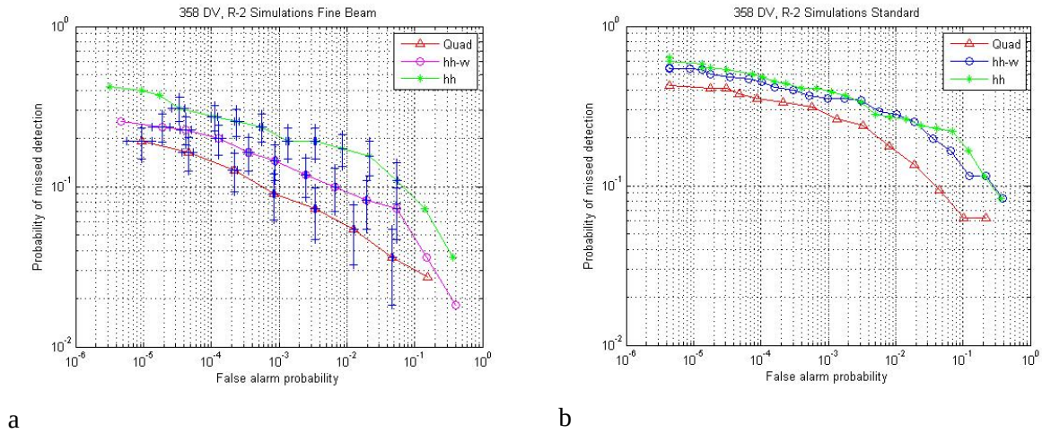
Figure 12: Detection performance for Dominion Victory (l41p1, 20 October 2005). a) Fine Quad-Pol Mode; b) Standard Quad-Pol Mode.
