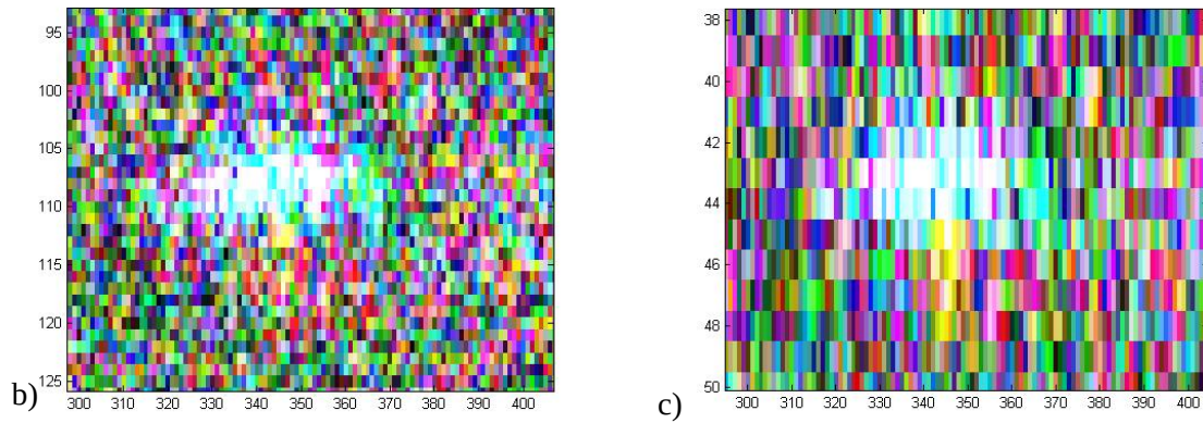
Figure 11: Polarimetric image of Dominion Victory (l41p1, 20 October 2005); a) CV-580; b) simulated RADARSAT-2 Fine Quad-Pol Mode; c) simulated RADARSAT-2 Standard Quad-Pol Mode.
