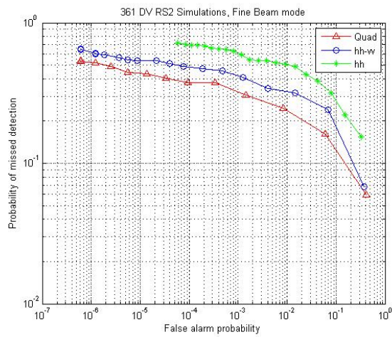
Figure 27: Detection performance for Dominion Victory (142p4, 20 October 2005). a) Fine Quad-Pol Mode; b) Standard Quad-Pol Mode.
