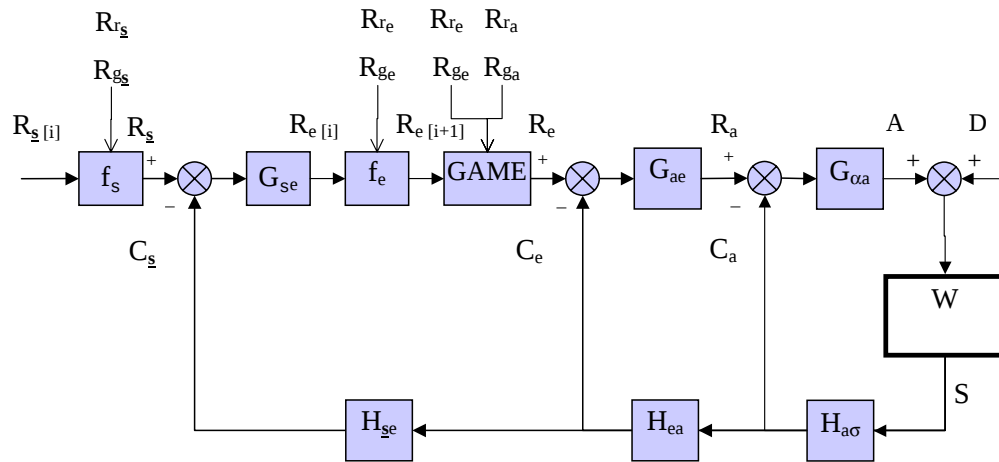
Figure 11: Simplified feedback control system model with serial feedback
