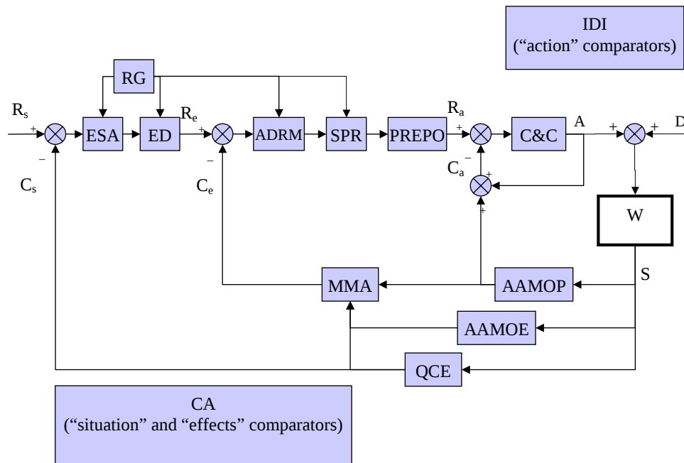
Figure 5: Feedback Control System model based on EBAO CONOPS v1.0.
