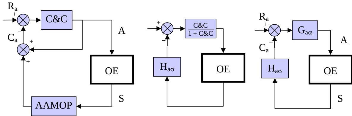
Figure 9: Simplifying the Action Loop
