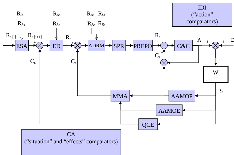
Note that the comparator that examines the desired and current situation variables is shifted to the right in Figure 6 compared to its position in Figure 5. That is, while the operation is proceeding, the current situation ( C_s ) would be compared to the most recent refined desired situation ( R_{s[i+1]} ). If the current situation were not converging onto the desired situation (i.e., EBAO control system is not stable) then this would trigger a re-examination of the strategic context and the initial desired situation.
