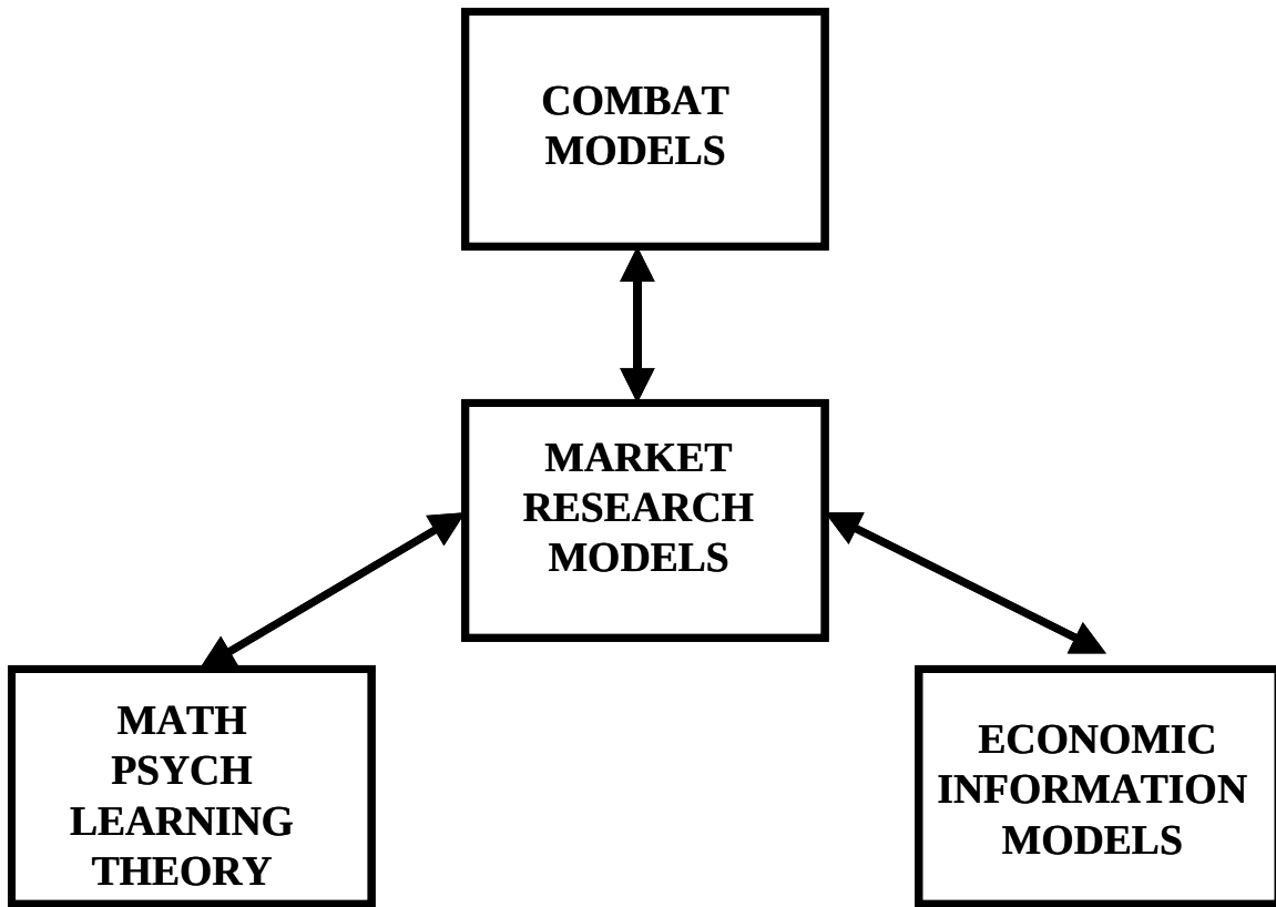
Figure 4.1 Project Structure
