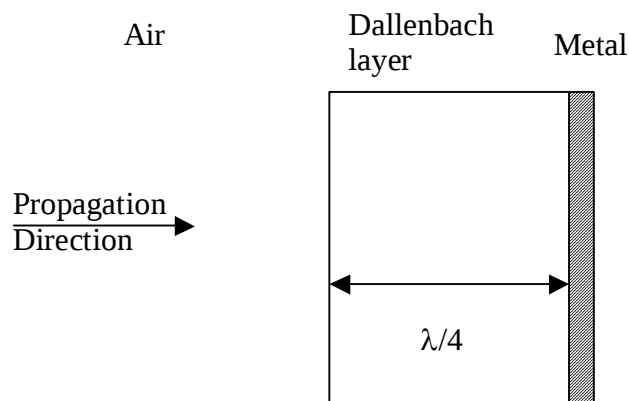
Figure 1: Dallenbach Layer.
