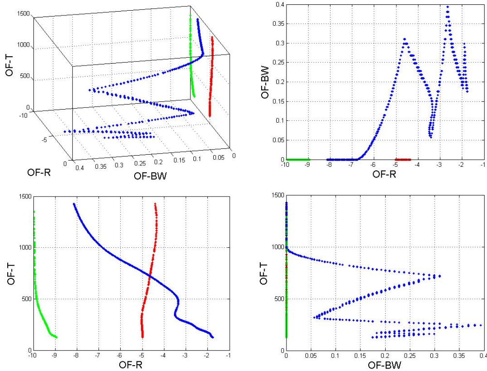
Figure 4: Plots of the objective functions for single layer Dallenbach absorbers made from materials 1 (green) 2 (blue) and 3 (red).
