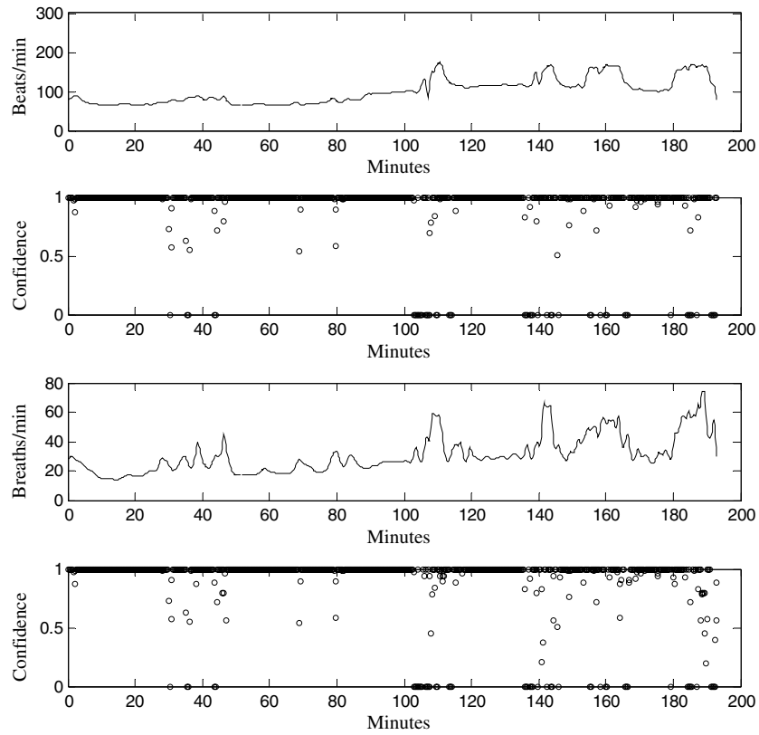
Figure 6. Heart rate and the corresponding confidence level (top two panels) along with RR and the corresponding confidence level (bottom two panels) for the same subject as in figure 5. The data were collected by the VivoMetrics system and were median filtered, resampled to 2 s intervals and filtered with a spline smoothing filter before application of the algorithm.
