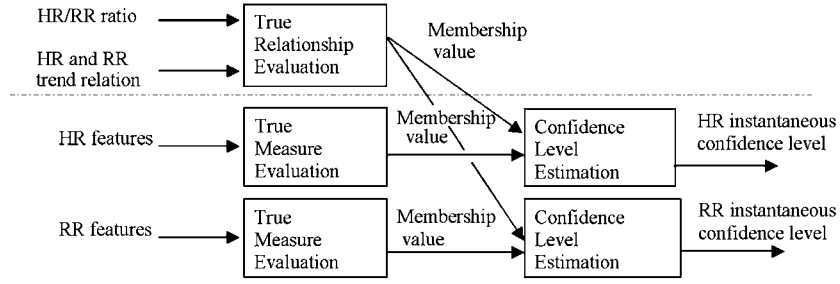
Figure 2. Block structure of the fuzzy logic algorithm to estimate confidence levels. The dotted line separates the parts of the algorithm that evaluate the relationships between the HR and RR (above the line) and the quality of the HR and RR measurements (below the line).
