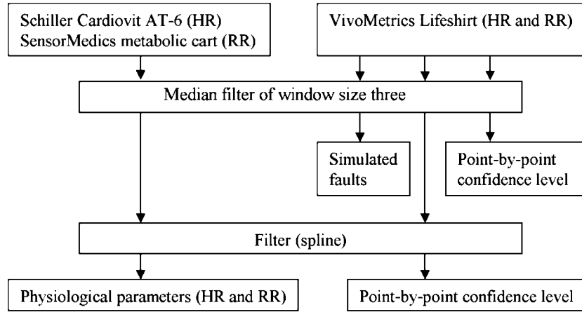
Figure 1. Datasets and processes used to develop and evaluate a fuzzy logic algorithm to assign confidence values to HR and RR.
