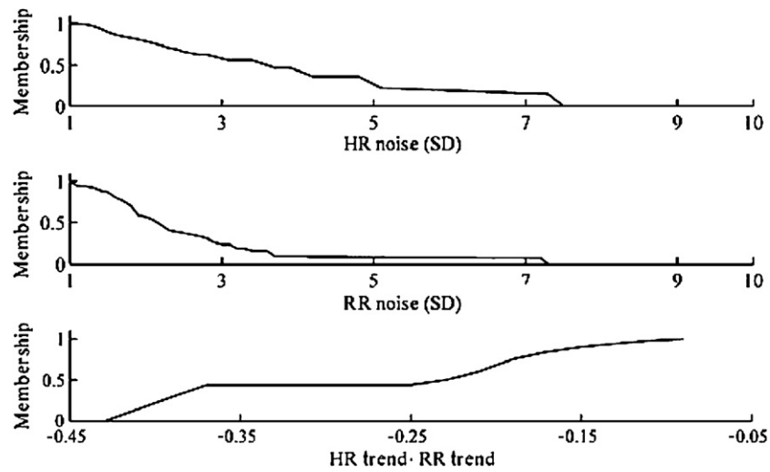
Figure 4. Data-driven membership functions for HR noise, RR noise and HR trend in beats per min/s ( \text{BPM s}^{-1} ) \times RR trend in breaths per min/s ( \text{BrPM s}^{-1} ).
