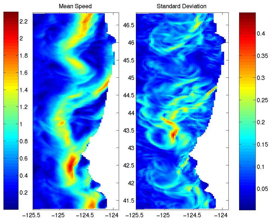
Figure 3: Speed of ensemble and time mean horizontal vector velocity ( m\ s^{-1} , left panel) and standard deviation of velocity deviations ( m\ s^{-1} , right panel) for a five-member ensemble of 60-day numerical simulations of wind-forced upwelling with perturbed initial conditions.
