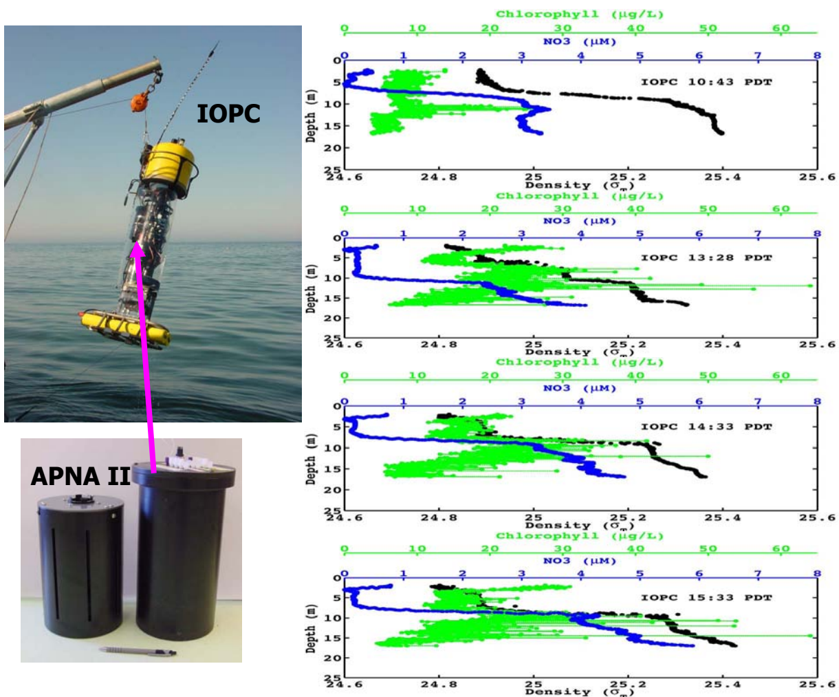
Figure 1. The IOPC profiler with the APNA II nutrient analyzer payload ready for deployment in Monterey Bay from the R/V Shana Rae and examples of hourly profiles for nitrate (blue), chlorophyll (green), and density (black) that were obtained autonomously with the system in Monterey Bay.
