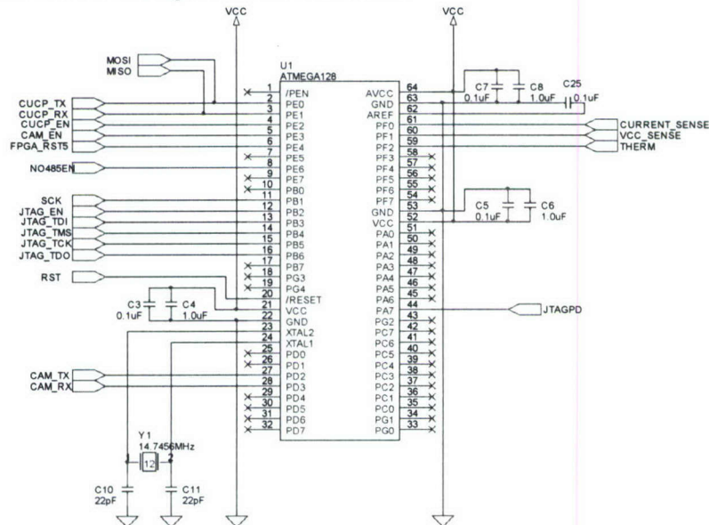
Figure 11 - CAM IB Microcontroller
