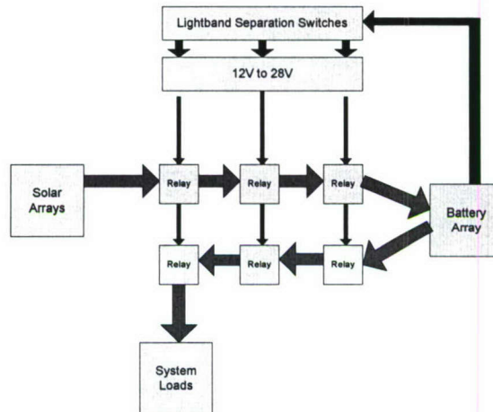
Figure 14 - Safety Inhibit Power Flow
