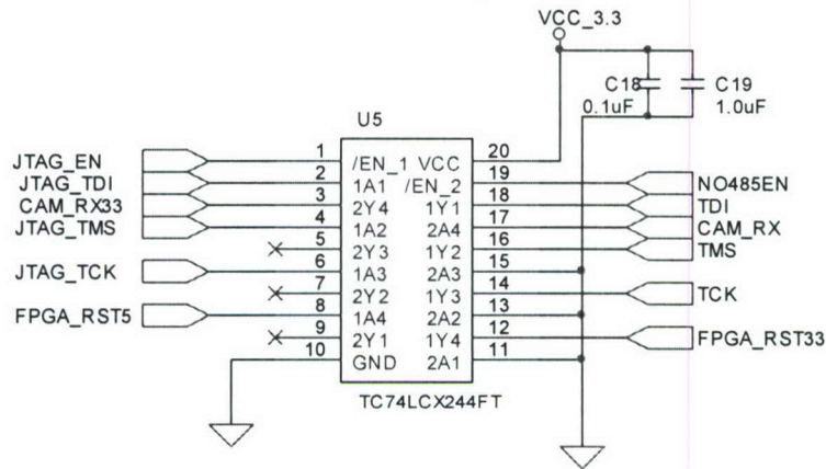
Figure 10 - CAM IB Level Converter
