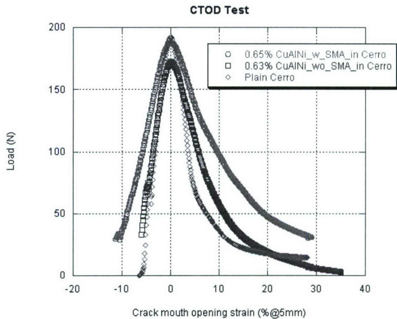
Figure 11. Load vs. crack mouth opening strain curves for fracture tests of three sample types: BiSn with heat treated CuAlNi particles, BiSn with unheat treated CuAlNi particles, and neat BiSn.
