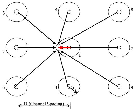
Figure 2. The configuration used for the cross-talk simulations. Red arrow represents signal, black arrows represent crosstalk, D is the channel spacing, and r is the distance between the center of the illumination bundle and that of the collection fiber within the same channel.
