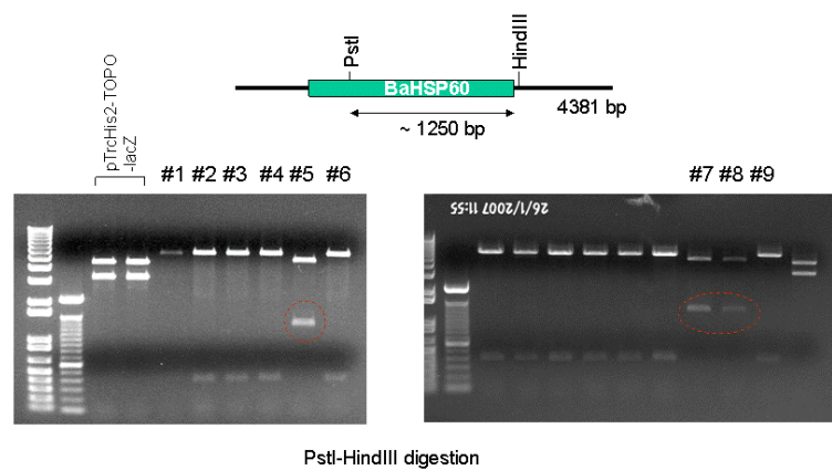
Fig. 41. Construction of BaHSP60 expression vector using pTrcHIS-2-TOPO vector.
