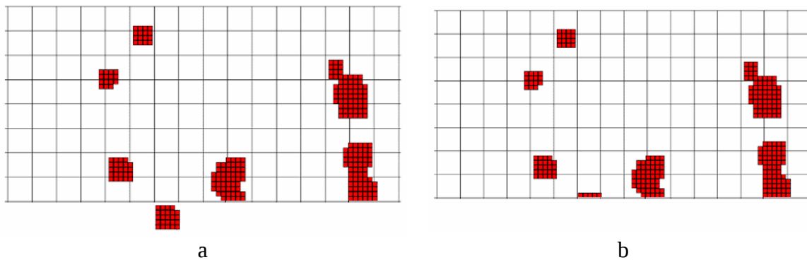
Figure 5. Reactive world model showing the placement of an obstacle off the map and behind the vehicle (a) and the resulting mirrored obstacle onto the map.
