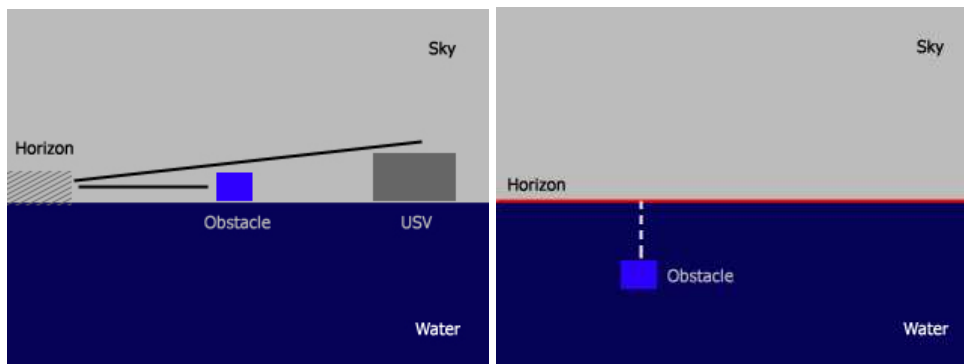
Figure 7. Trigonometric calculations of range of an obstacle
