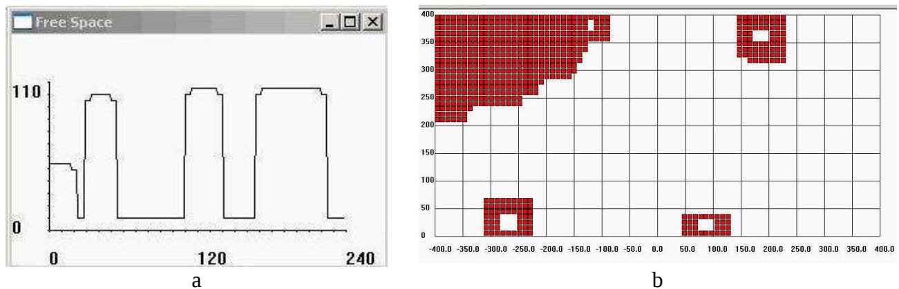
Figure 6. Free space voting behavior with decrease in value for near-obstacles (a) and the corresponding obstacle map (b)
