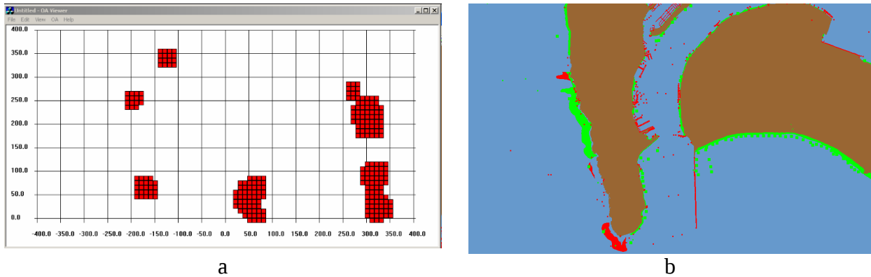
Figure 2. World model obstacle maps used by the reactive OA (a) and the deliberative OA (b)
