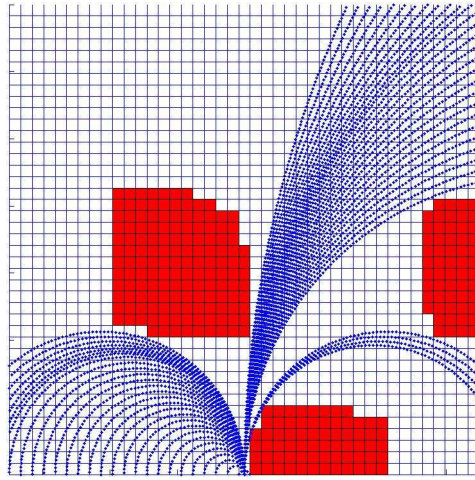
Figure 4. Reactive world model with obstacles and possible arc paths
