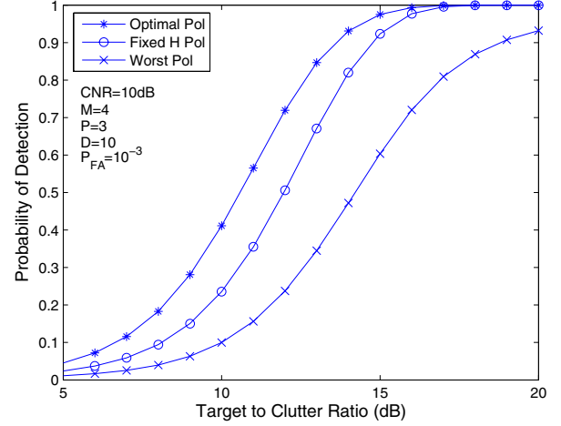
Fig. 4. Detection performance of the GLR test statistic T_{GLR} as a function of the target-to-clutter ratio, for P_{FA} = 10^{-3} .
