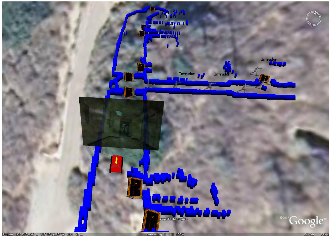
Figure 3. Overlay of the robot's mapping, door finding, and intruder detection perceptions from the interior of an underground World War II bunker on Google Earth.
