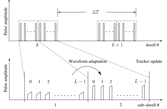
Fig. 1. Pulse diagram of the proposed adaptation algorithm. The pulse amplitudes are for illustrative purposes only.
