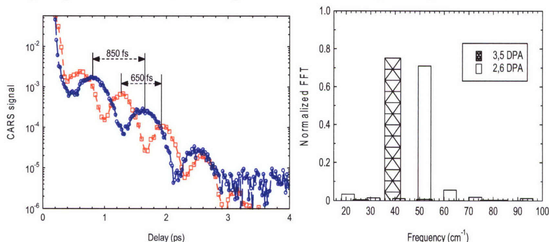
Fig. 7. Left: CARS signals at 1400\text{ cm}^{-1} as function of probe delay for 2,6-DPA (squares) and 3,5-DPA (circles) solutions in \text{H}_2\text{O}/\text{KOH} . The signals are normalized to the peak of the four-wave-mixing signal. Right: Fourier transforms of the time-delayed CARS data for 3,5-pyridinedicarboxylic acid (shaded) and 2,6-pyridinedicarboxylic acid (empty).
