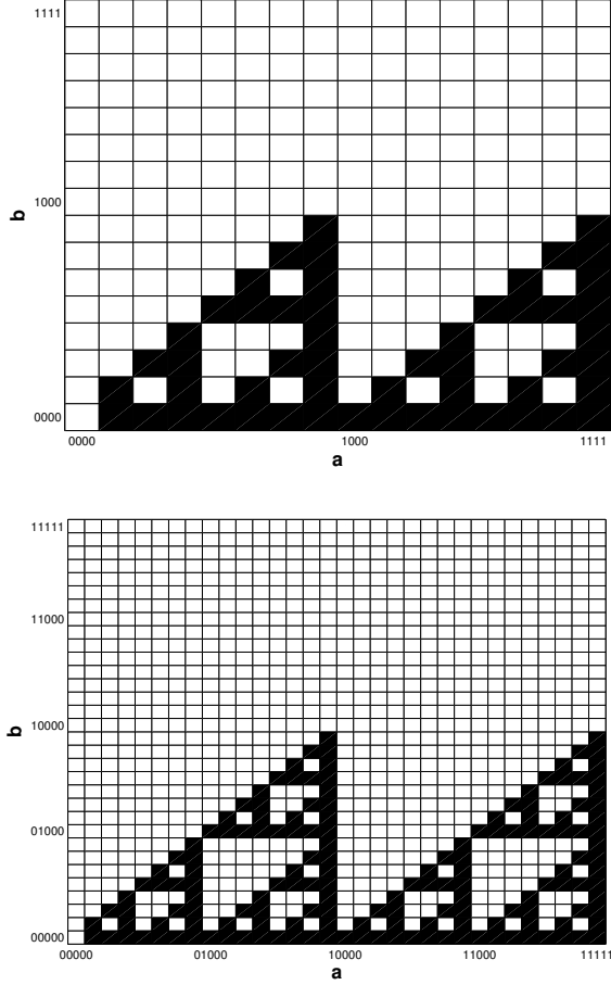
Figure 1: Supports of the subspace S_\Delta for m = 4 and m = 5 .
