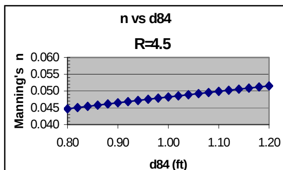
Figure 4. Variation of Manning's n value with sediment size using Limerinos' Equation – Moose River, NH.
