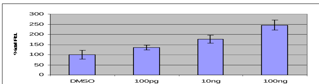
Figure 1 Estrogen induces ROS formation in MCF-7 cells in dose dependent manner as assayed by DCFDA oxidation. MCF-7 cells (5000 cells/well) were growth synchronized by culturing it in growth media w/o serum for 48hrs post seeding. DCFDA were loaded with 10uM for 20mins after which cells were exposed to various concentration of E2 and emissions read at 10mins post treatment on fluorescence plate reader. The level of ROS is expressed as relative fluorescence unit and vehicle (DMSO) treated value was considered 100%.
