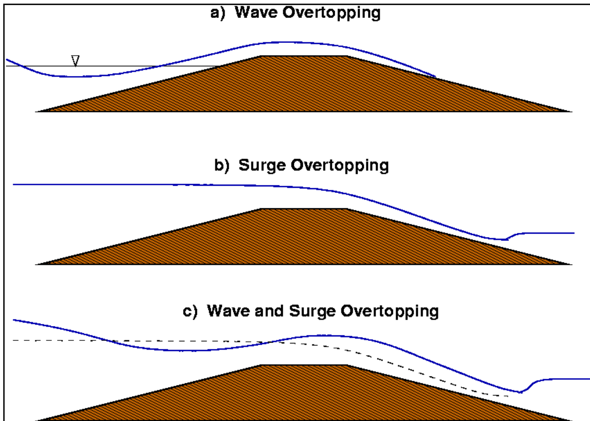
Figure 1. Overtopping scenarios for earthen levees.
