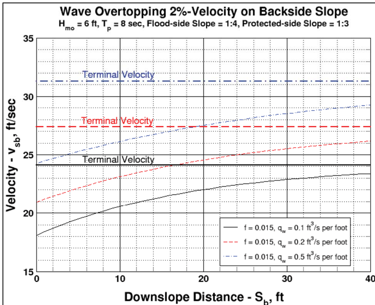
Figure 3. Wave overtopping flow velocity on protected-side slope.
