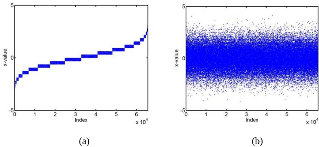
Fig. C4. Comparison of (a) ordered and (b) shuffled values.
