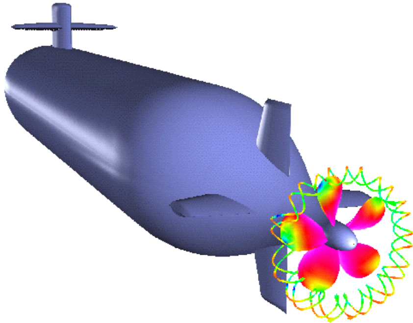
Vortex Ring Produced by the Crashback Maneuver
