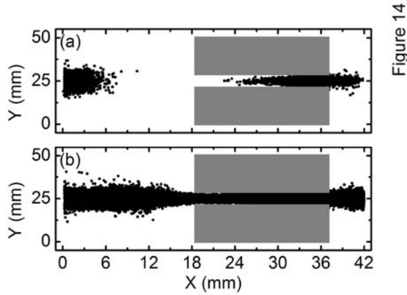
FIG. 14. Argon X - Y phase space for a hollow cathode depth D = 18.5\text{ mm} , hole height h = 8\text{mm} and the seed electrons are injected with an average energy equal to the ionization peak for the times (a) 25\text{ ns} and (b) 38.5\text{ ns} , where the electron peak current is achieved at 38.5\text{ ns} . The gray boxes indicate the hollow cathode face.
