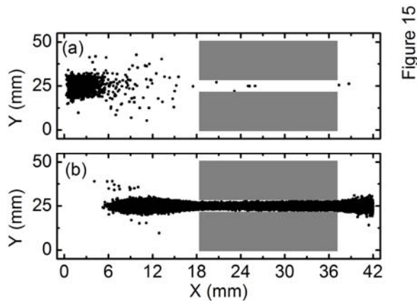
FIG. 15. Electron X - Y phase space for a hollow cathode depth D = 18.5\text{ mm} , hole height h = 8\text{mm} and the seed electrons are injected with an average energy equal to the ionization peak for the times (a) 25\text{ ns} and (b) 38.5\text{ ns} , where the electron peak current is achieved at 38.5\text{ ns} . The gray boxes indicate the hollow cathode face.
