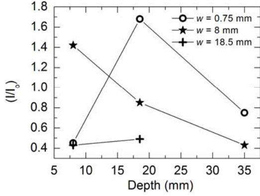
FIG. 10. The variation in the peak electron current arriving at the anode with the hollow cathode depth, D , and thickness, w , where I_0 is the peak current for D = 8 mm, w = 0.75 mm, h = 8 mm and 1 keV seed electrons, the hole height h = 8 mm and the seed electrons are injected energies up to 2.5 eV.
