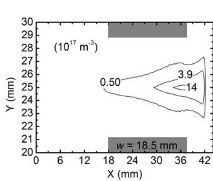
FIG. 12. Argon ion density for a hollow cathode depth D = 18.5 mm, hole height h = 8 mm and the seed electrons are injected with energies up to 2.5 eV at the time 1016 ns, where the electron peak current is achieved at 1017 ns.
