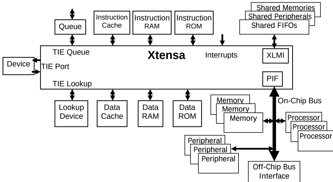
Figure 5 Xtensa Interfaces
