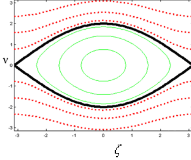
Figure 7. Separatrix and orbits on a pendulum phase space diagram.
