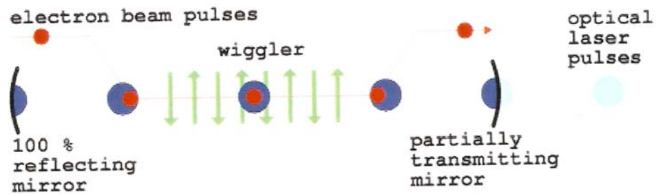
Figure 5. Schematic of a resonator from [3].
