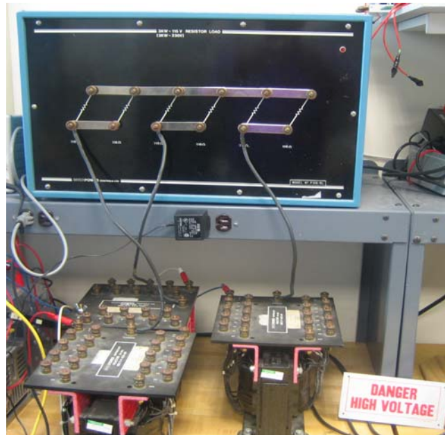
Figure 28. Load Components.
