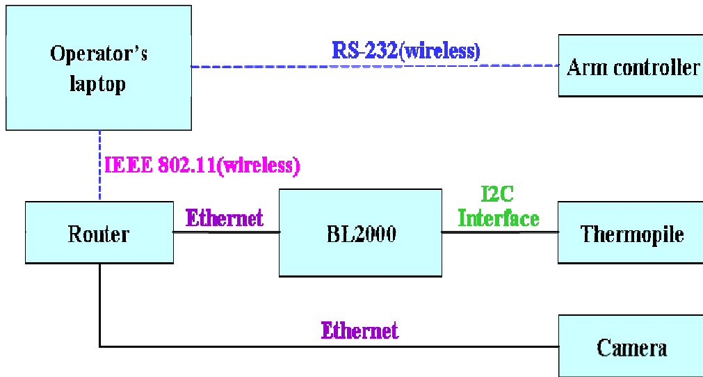
Figure 13. Block Diagram for the Arm, Camera and Thermopile.
