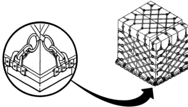
Figure 9. 463L Pallet.
