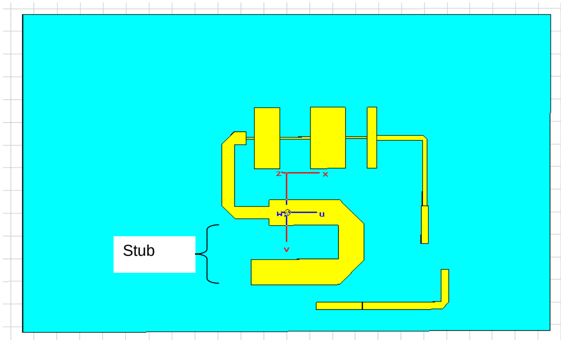
Figure 41. Rectenna Circuit Showing the Front End Matching Stub.
