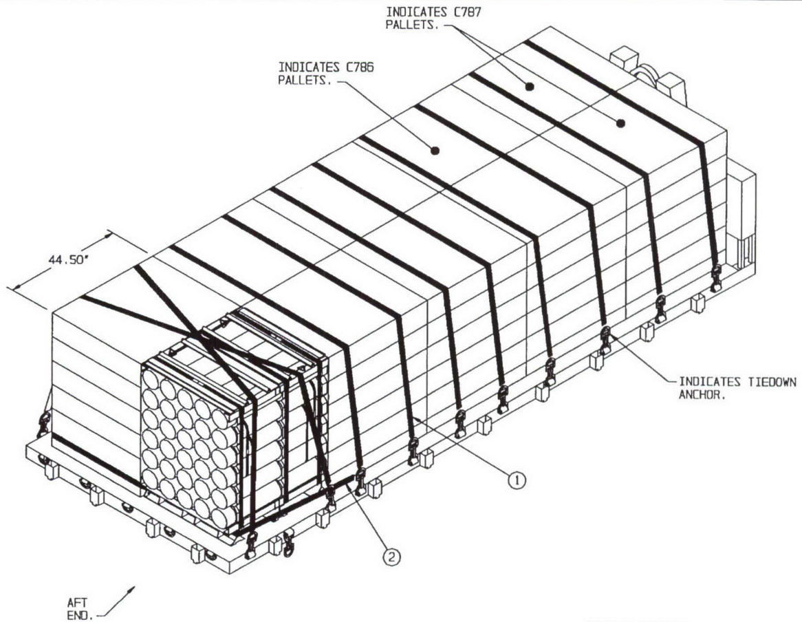
ISOMETRIC VIEW
