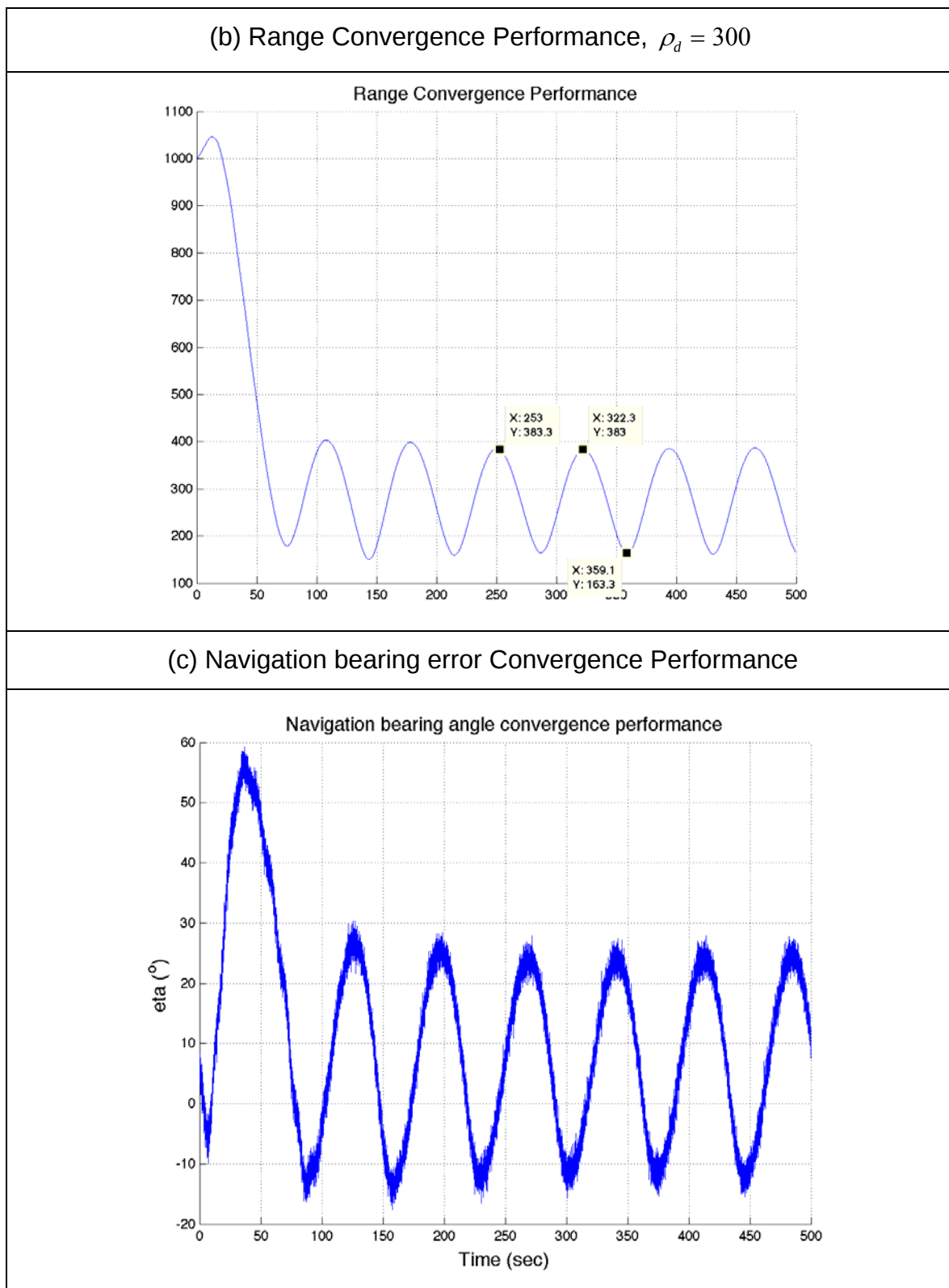
Figure 33. Non-Maneuvering Target Tracking Performance with Gain k_1 = 0.05
