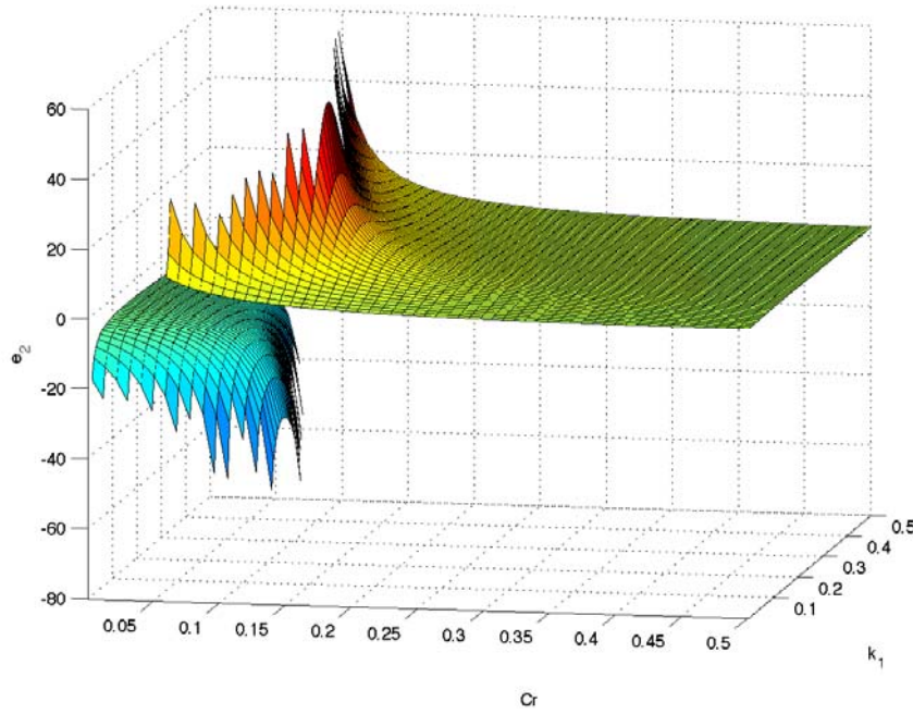
Figure 5. Moving Target case, e_2 = f(k_1, c_\rho) for v_g = 10 , v_t = 10 , \rho_d = 100
