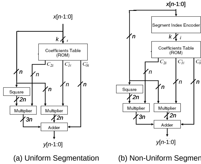
Figure 48 Basic Quadratic NFG Architectures. (After [8])
