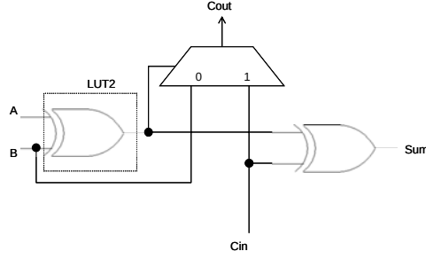
Figure 19 Single-bit Full Adder Implemented on Virtex-II FPGA.
