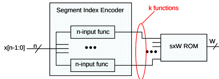
Figure 33 Generic Address Encoder.
