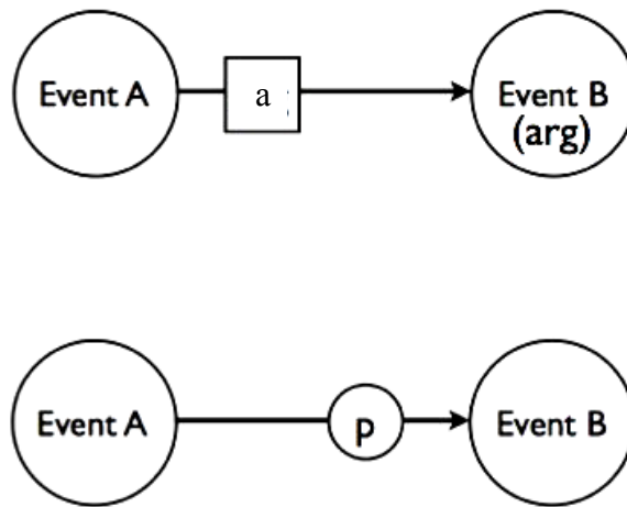
Figure 9. Special cases of Event Graph notation. (After: Buss, 2001.)
