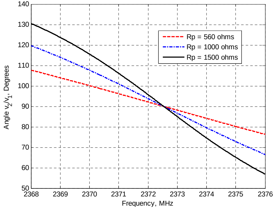
Figure 31. Angle of \frac{v_2}{v_1} plot at R_p = 560 \Omega , 1000 \Omega and 1500 \Omega .
