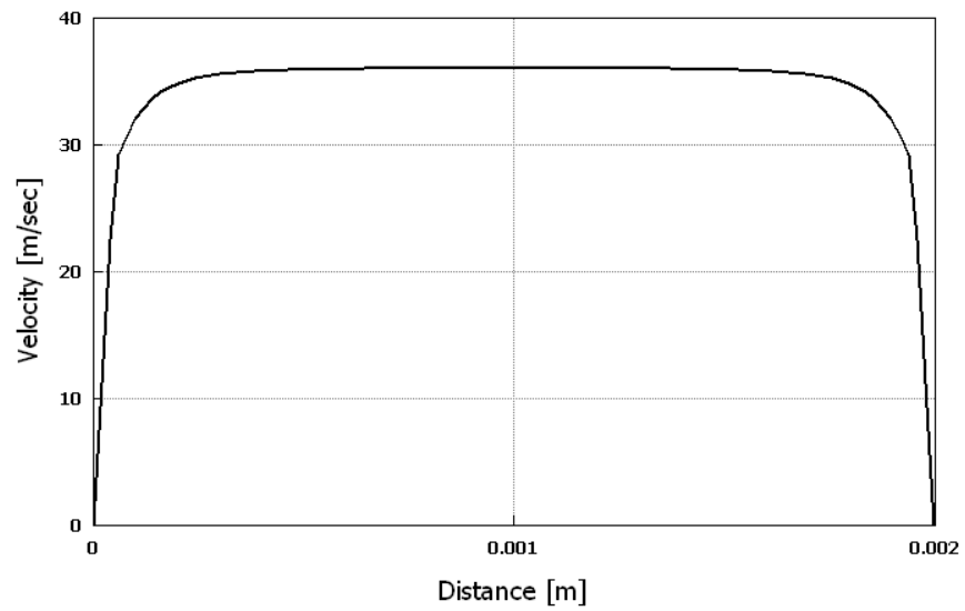
Figure B5. Velocity profile at x = 0.01
