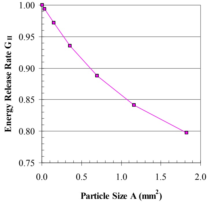
Figure 17. Energy release rate G_{II} for reinforcing particle b in matrix material of composite plate varying particle size from A=0.01mm^2 to A=2mm^2 with particle stiffness E_3 = 400GPa at prescribed distance r = 1.124mm to crack tip.
