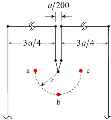
Figure 13. Composite plate matrix material containing reinforcing particles a , b , c in position radial distance r to crack tip.
