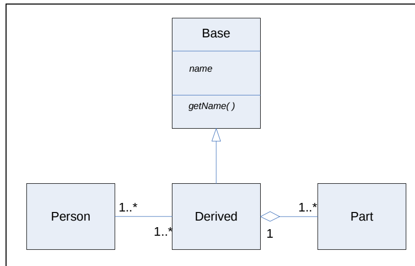
Figure 12 Class diagram
