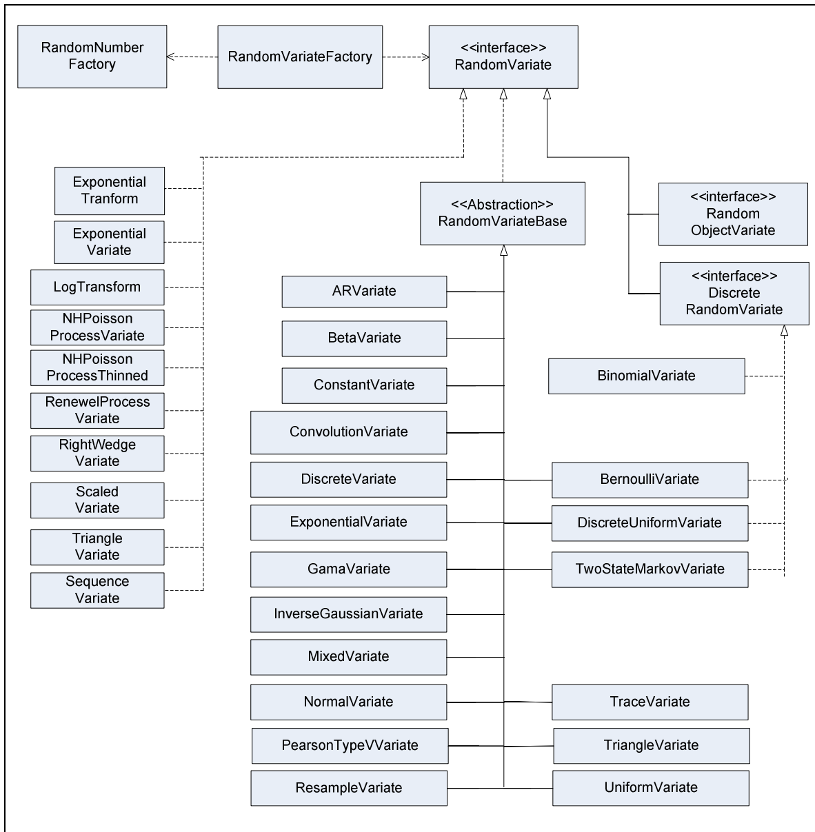
Figure 54 Existing Simkit.Random package, All Random-Variate Classes
