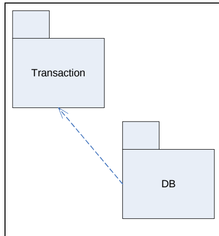
Figure 13 Package diagram
