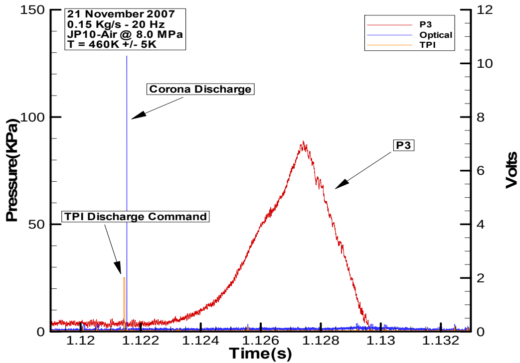
Figure 35. Successful JP-10/air Ignition for \dot{m}_{air} = 0.15 kg/s
