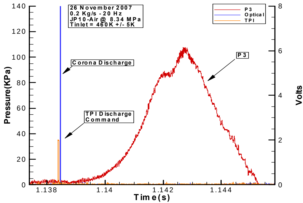
Figure 36. Successful JP-10/air Ignition for \dot{m}_{air} = 0.2 kg/s
