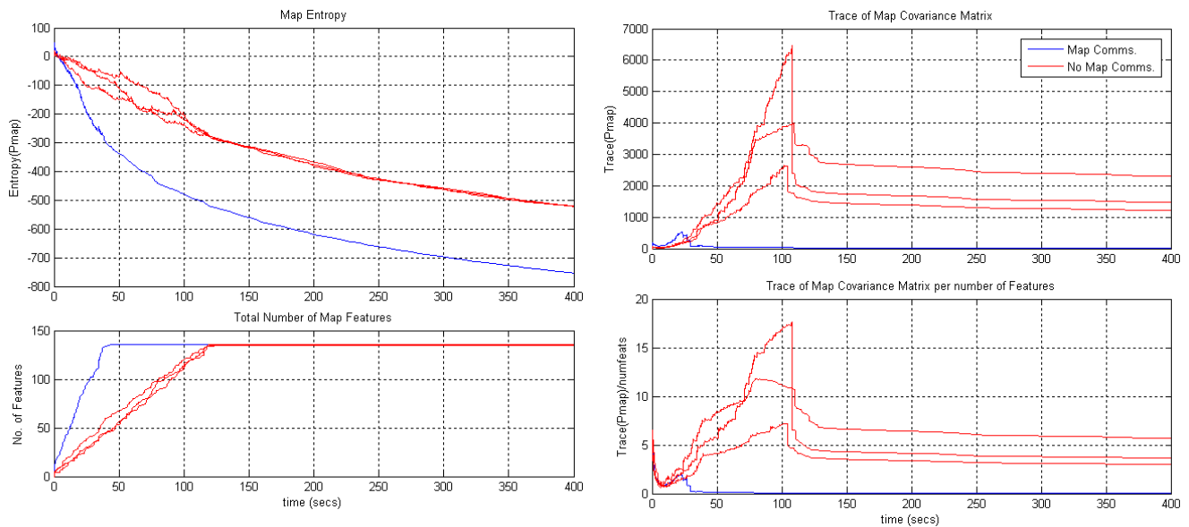
Fig. 11. Multi-UAV SLAM (Big Triangle Trajectory): Entropy, map size, covariance trace and covariance trace per feature number comparison for runs with map information communication and for runs with no map communication.
