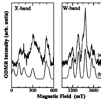
FIG. 7. (a) Experimental ODMR spectra from \text{GaN}_{0.018}\text{P}_{0.982}/\text{Si} , taken at 5 K at both the X (9.31 GHz) and W (94.8 GHz) bands. (b) The simulated ODMR spectra for \text{Ga}_i\text{-B} .
