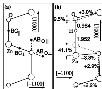
FIG. 1. (a) Schematic representation of the four H sites in ZnO and (b) calculated atomic positions for \text{H}^+ at the \text{BC}_{\parallel} site, in the (11–20) plane. The dashed circles and dashed lines indicate bulk atomic positions and bonds, respectively. Distances are given in unit of Å and percentage changes are with respect to the bond length of bulk ZnO.
