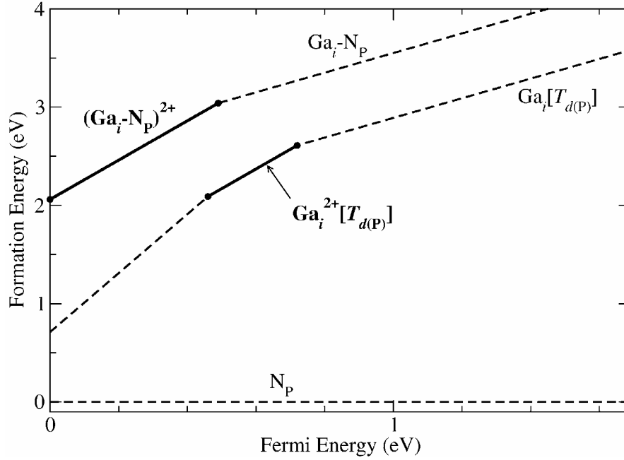
Fig 9. The formation of Ga_i-N_P complex. The charge states with an unpaired electron are plotted with thick solid lines with boldface labeling including the charge state numbers. The chemical potential of the N atom is set such that N_P has zero formation energy.
