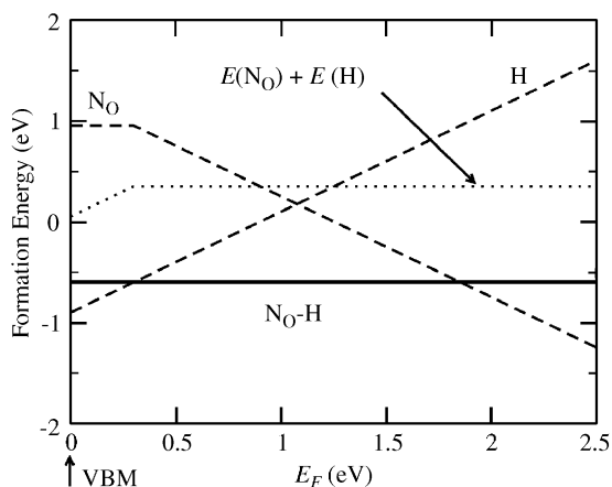
Fig. 3. Formation energy of an interstitial H, N_O (dashed lines) and a N_O –H complex (solid line) in ZnO as a function of electron Fermi energy. The dotted line shows the sum of the formation energies of an isolated interstitial hydrogen and an isolated N_O . The Zn-rich condition, N_2 and H_2 phase precipitation limits were assumed. The energy difference between the dotted line and the solid line is the binding energy of the N_O –H complex.
