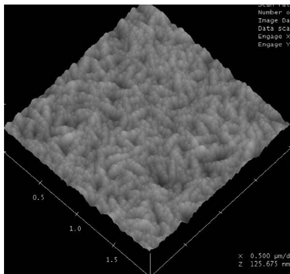
Fig. 1. The topography of a 0.74- \mu\text{m} -thick ZnO:N film grown on a glass substrate at 400 ^{\circ}\text{C} .
