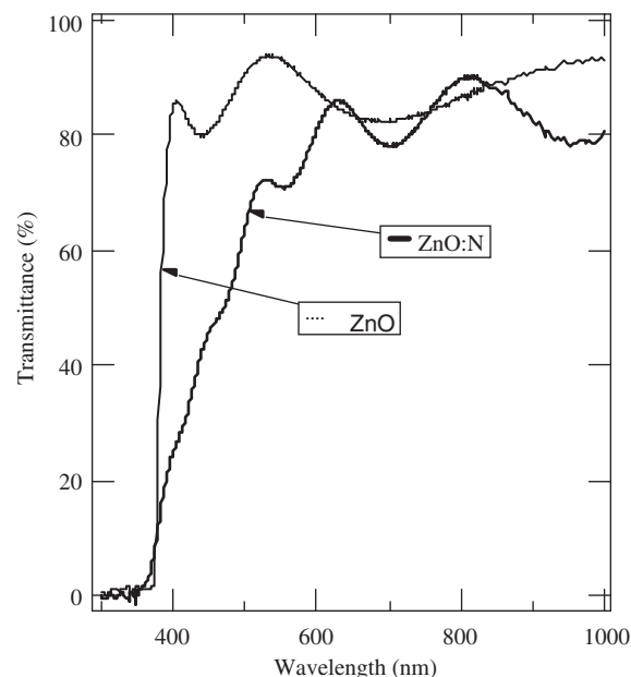
Fig. 3. Optical transmittance of ZnO and ZnO:N films. Both films were deposited on glass substrate at 400 ^{\circ}\text{C} .
