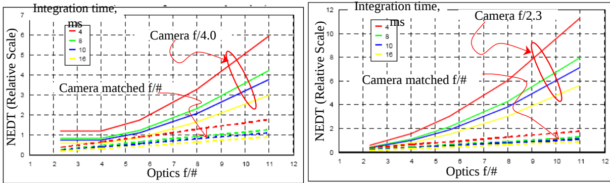
Figure 12. NE \Delta T for a f/4 camera (left), and f/2.3 camera (right): scene = 290K, optics 300K, @3 \mu m (several T_{\text{intg}} ); solid lines show camera fixed f/\# ; dashed lines show camera with CVA/CS, constantly matched to optics f/\# (NE \Delta T is better if it is a smaller number).
