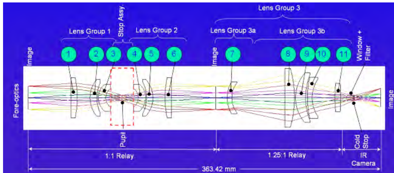
Figure 3. Optical relay with an external cold CVA/CS assembly.
