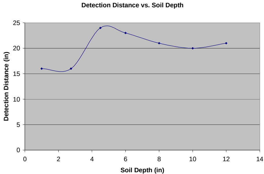
Figure 43. AWID tag detection range (directly above tag) as a function of soil overburden depth.
