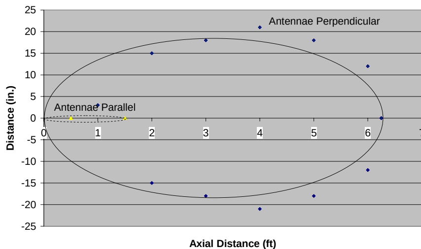
Figure 49. Detection results for the modified Trolley Scan RF Tag System (copper pipe in air)
