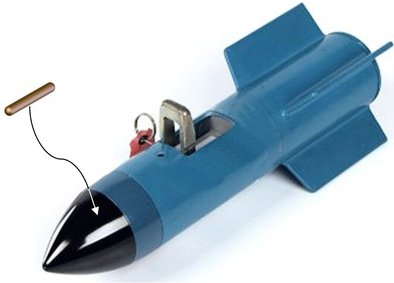
Figure 10. Option 1 for mounting tag in nose of MK-52
