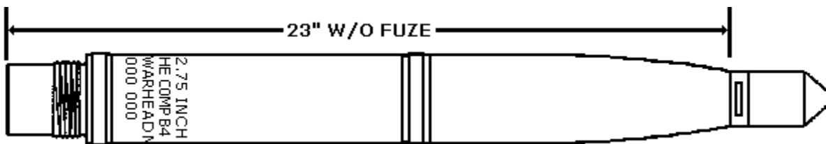
Figure 21. M229 HE warhead
