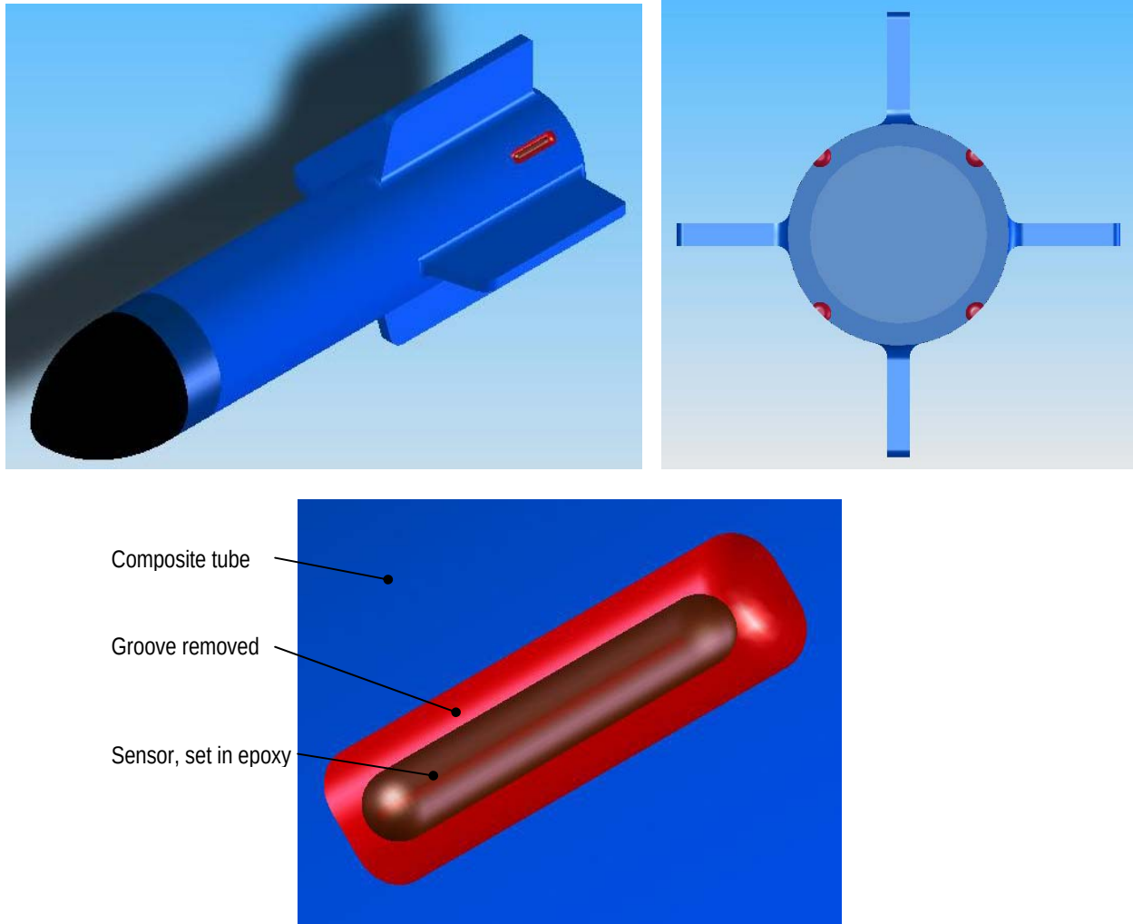
Figure 11. Option 2 mounting tags in MK-52 main body near tail
