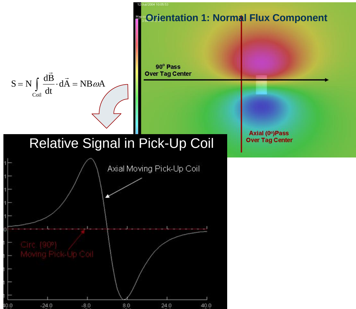
Figure 31. Sample calculation of the voltage in a pickup coil as the coil is moved past the tagged target. The false-color units of the upper-right plot are Tesla per Amp-Turn. The vertical units in the bottom plot are relative to voltage levels. Absolute values are not available because the transmitted field is in Tesla per Amp-Turn. The horizontal values in the lower plot are inches with the zero inch value being the above-ground coil directly over the center of the ordnance item
