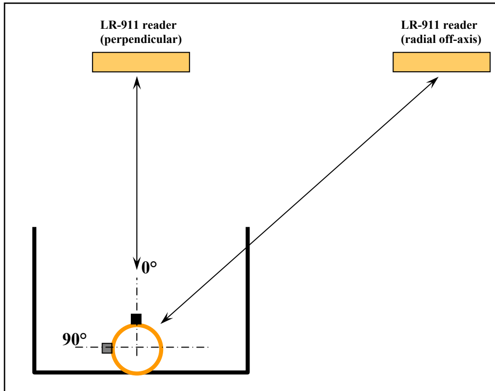
Figure 41. Measurement geometry for determination of maximum AWID tag range in soil. The pipe is rotated over a 90 degree range for these measurements. In the 90 degree orientation, the copper pipe shields the tag from the reader.
