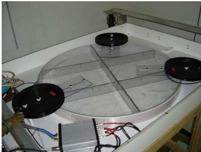
Figure 2. View of the above-ground detection equipment showing the one-meter diameter transmit coil and the three independent detection coils
