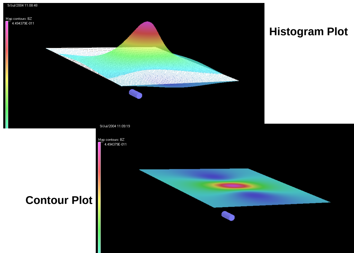
Figure 30. Peak amplitudes at location 15 inches above tag with munition oriented parallel to surface is about 50 pT per Amp-Turn
