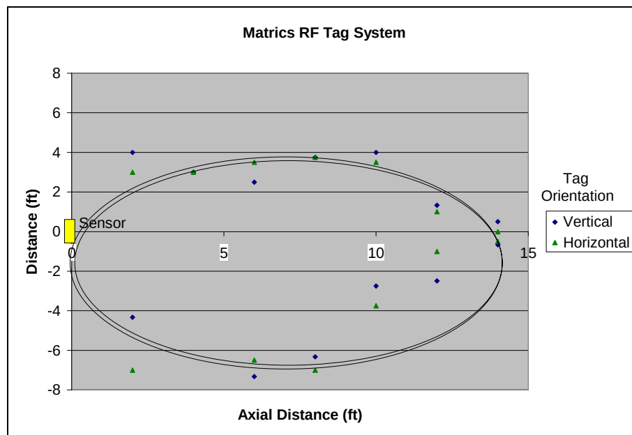
Figure 54. Laboratory measurement of tag range and azimuth angle of Matrics tags
