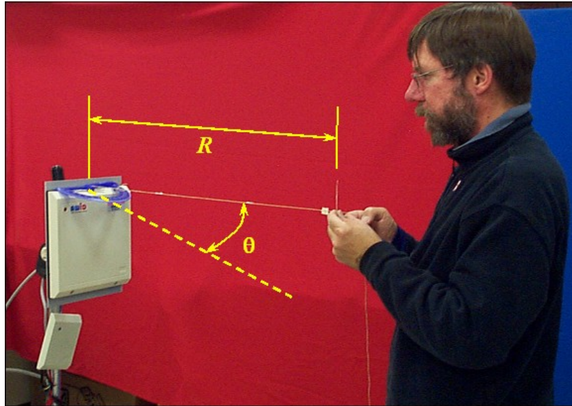
Figure 38. Laboratory geometry for AWID UHF tag evaluation
