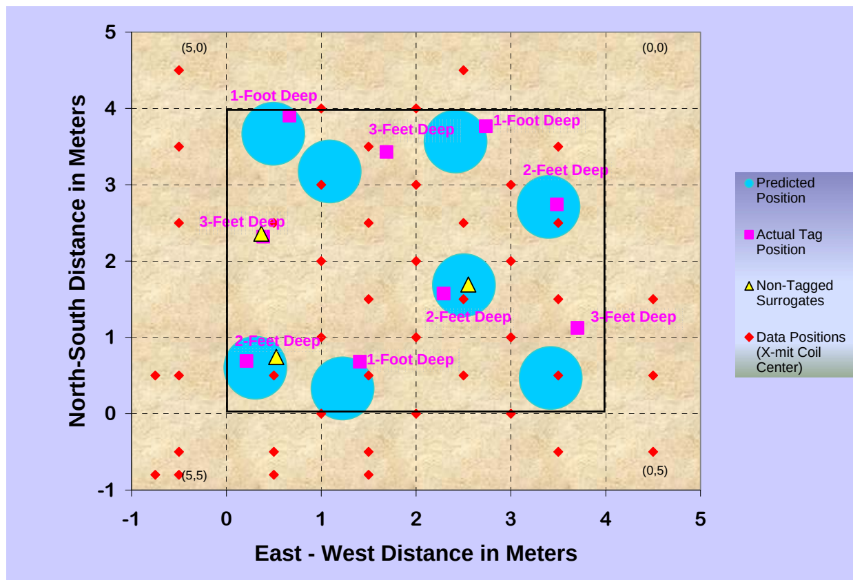
Figure 93. Plan view of the test grid at Aberdeen Test Center showing the actual tagged munition positions, Battelle's predicted positions, and the positions where Battelle acquired data
