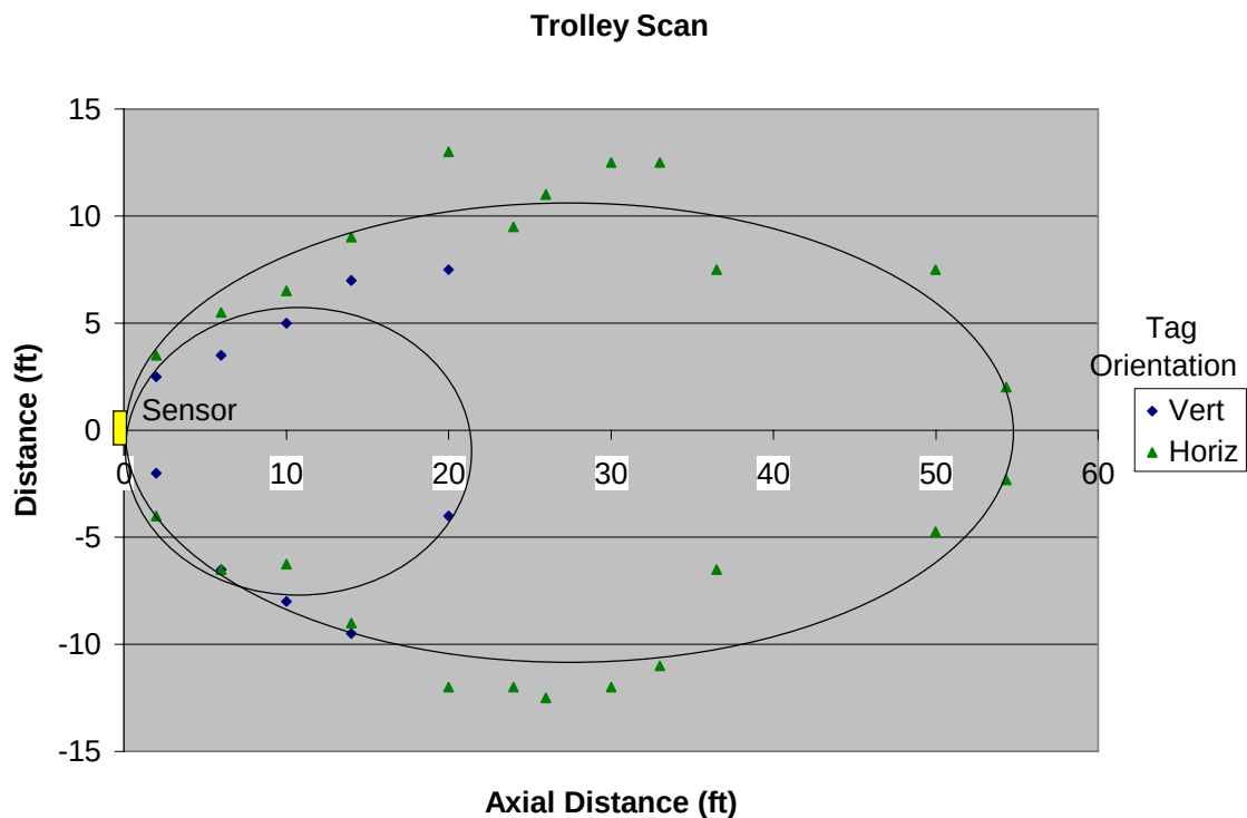
Figure 47. Laboratory measurement of tag range and azimuth angle with the Trolley Scan tags
