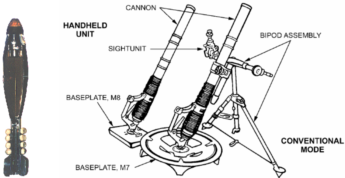
Figure 13. 60mm cartridges
