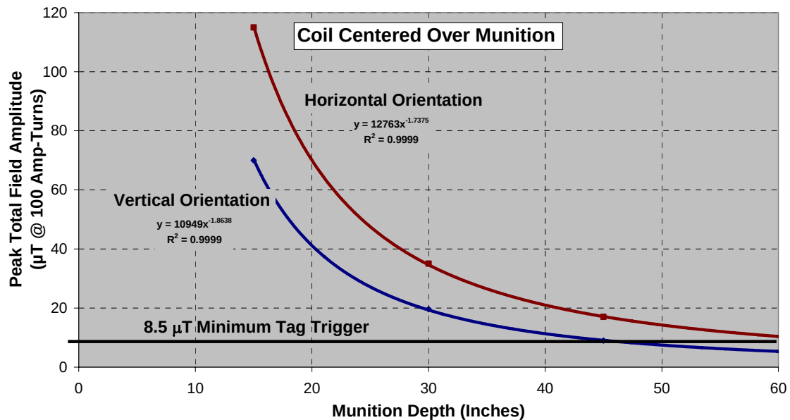
Figure 25. Magnetic field on the surface of a munition versus depth in the ground for realistic interrogating signal strength (vertical and horizontal munitions)
