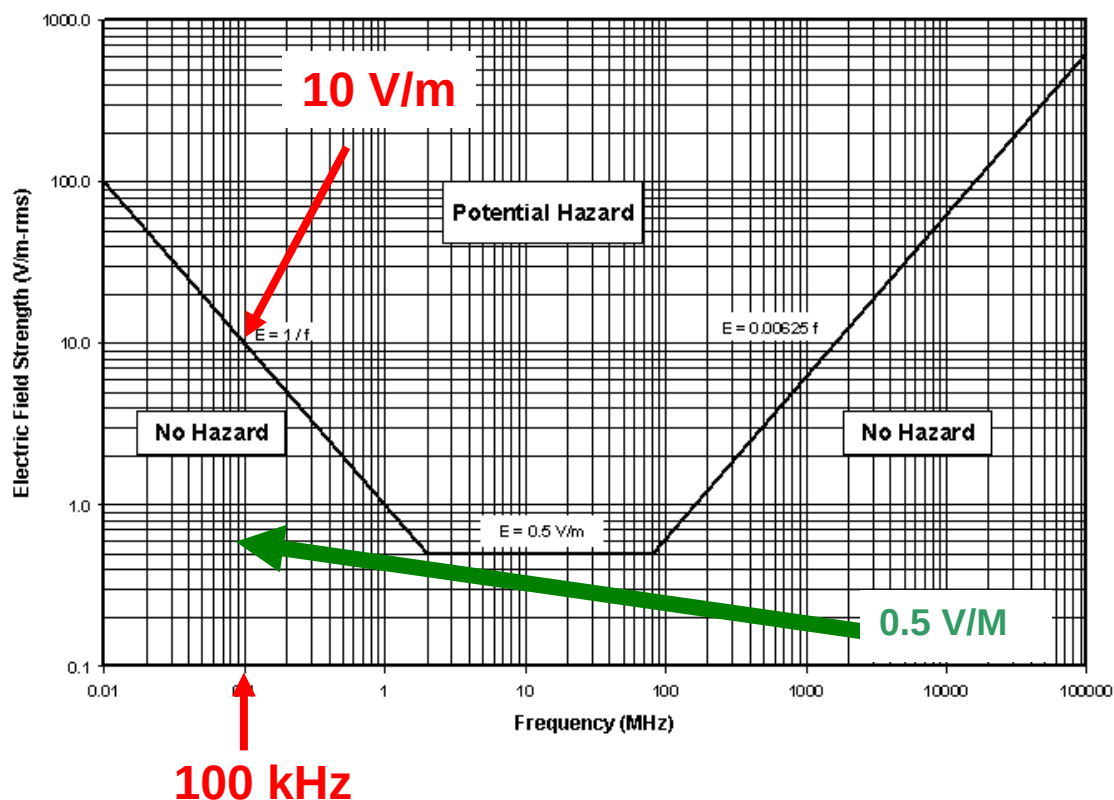
Figure 88. HERO safety levels and the theoretical value of the Battelle one-meter diameter interrogating coil
