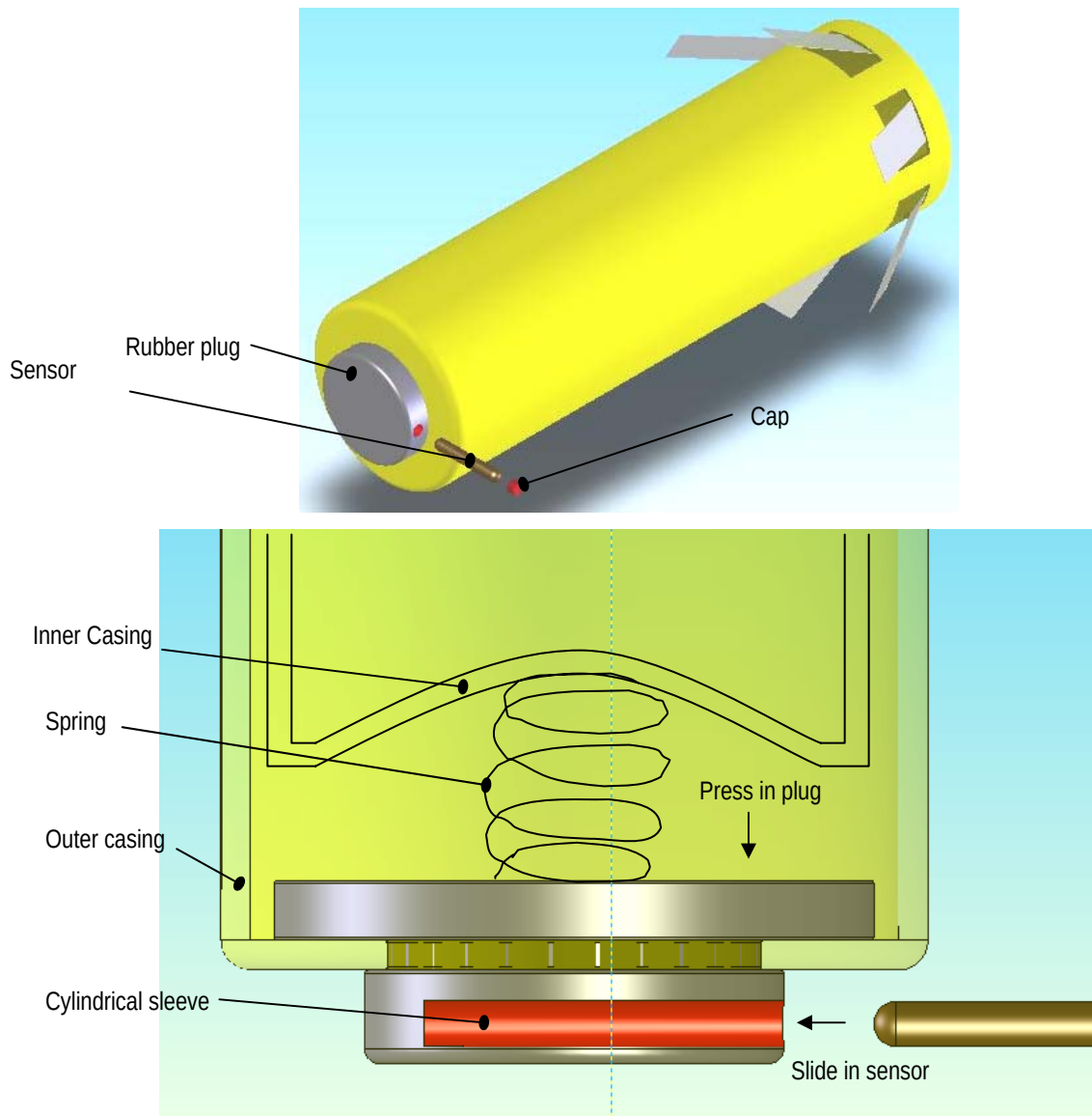
Figure 7. Mounting Option 2 for BLU-97
