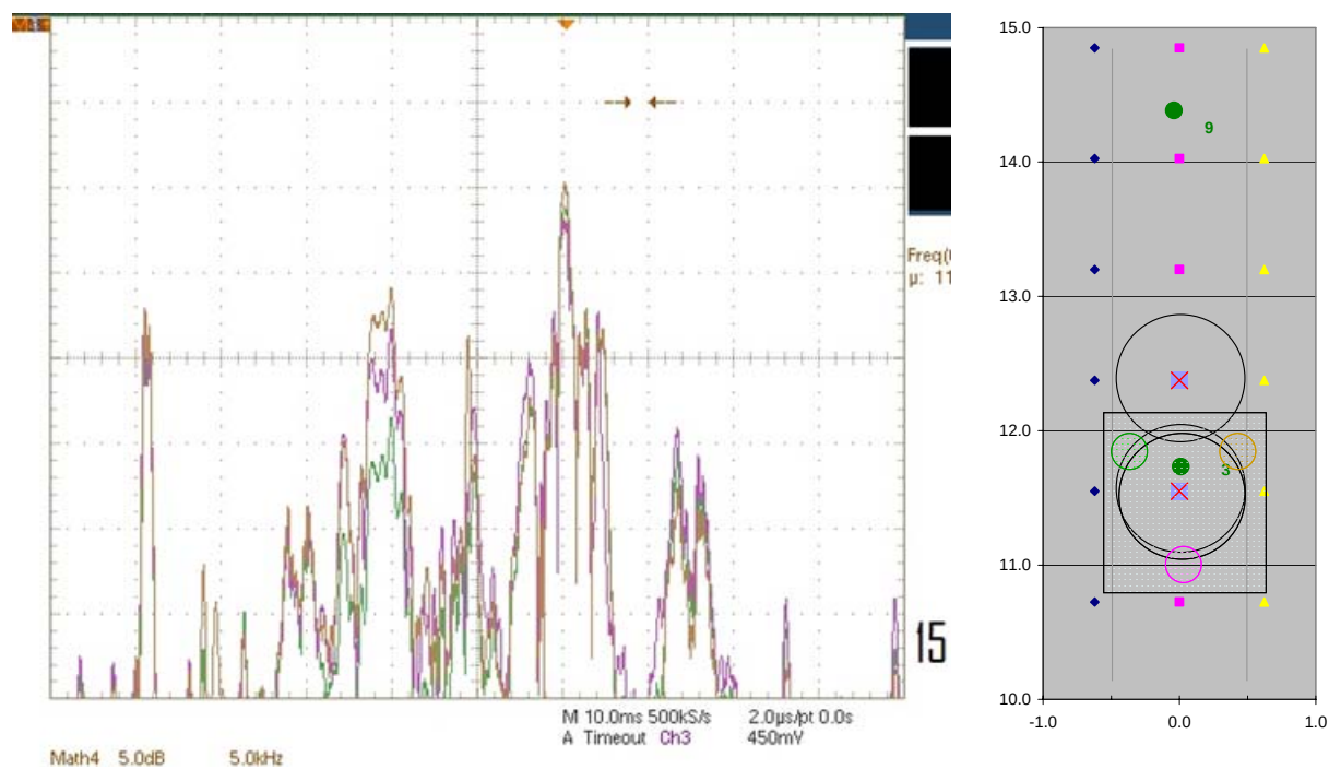
Figure 85. Data taken at point (15, C), above surrogate 3, which is buried 3 feet beneath the surface
