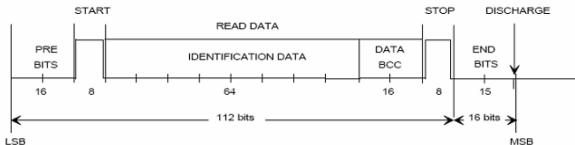
Figure 35. Texas Instruments' depiction of the tag's reply message
