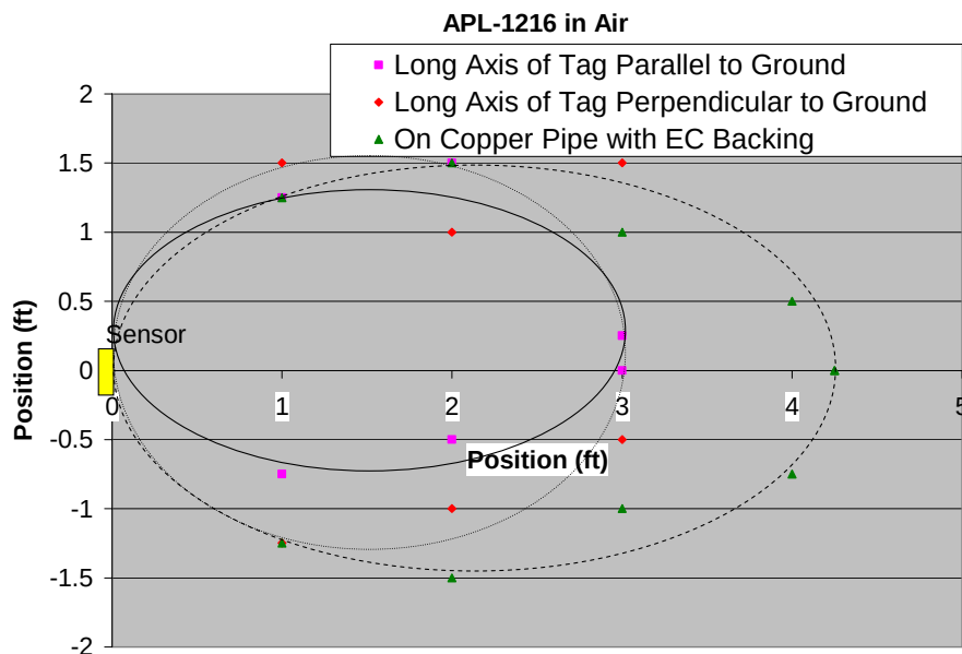
Figure 66. Detection distance of APL-1216 in air with the EC material backing
