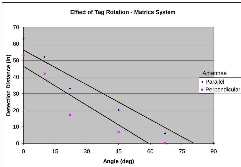
Figure 57. Matrics tag detection range as a function of orientation of copper pipe
