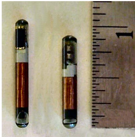
Figure 4. Two sizes of the Tiris solenoidal tags
