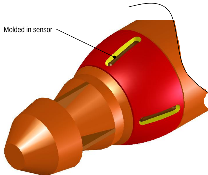
Figure 16. 60mm cartridge Option 2
