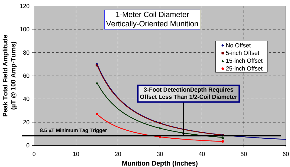
Figure 26. Magnetic field on the surface of a munition versus depth in the ground for realistic interrogating signal strength, a vertically-oriented munition, and coil center offsets of zero, 5 inches, 15 inches, and 25 inches.
