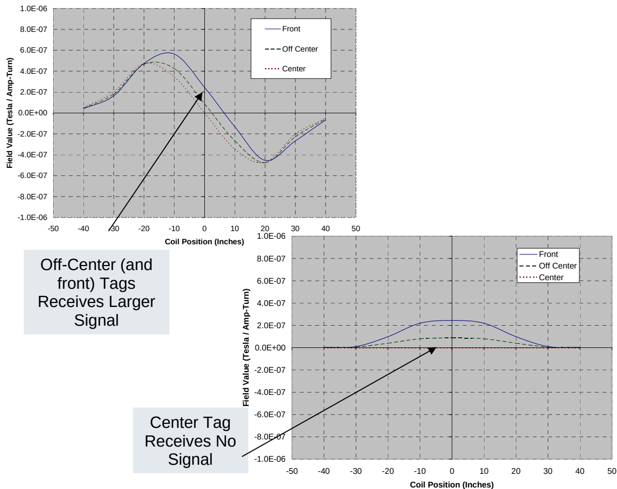
Figure 29. Responses calculated as the interrogating coil moved past the munition, in the simulation of a UXO search procedure. The left curve corresponds to the search coil moving parallel to the axis of the horizontal munition and the right curve corresponds to the coil moving perpendicular to the munition's cylindrical axis.
