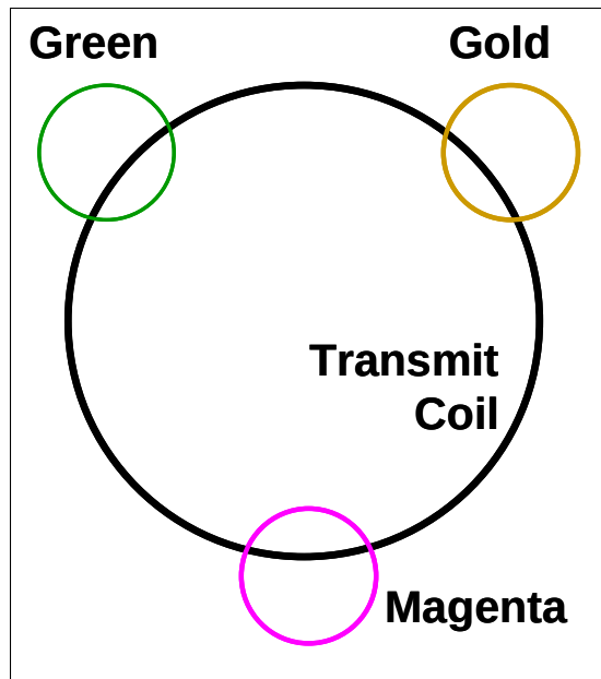
Figure 96. This drawing depicts the arrangement of the three receive coils in the above-ground coil module. The alignment of the coils is in the same heading as Figure 95. The colors of the receive coils match the colors in the data plots. Subsequent figures include this drawing positioned over the grid location where the data set was acquired.
