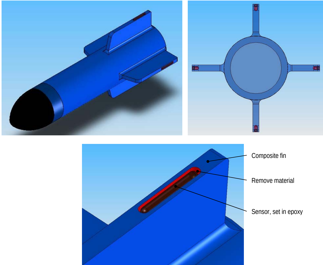
Figure 12. Mounting tag in MK-52 fins, Option 3
