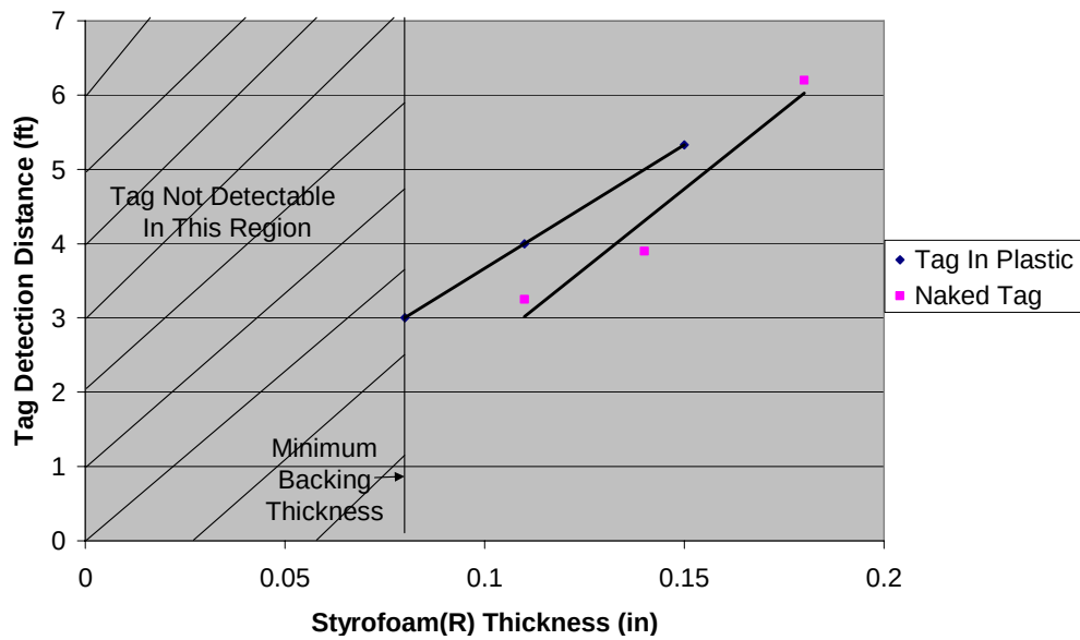
Figure 61. Detection distance as a function of Styrofoam® backing thickness when Trolley Scan RF tag is placed on a conductor
