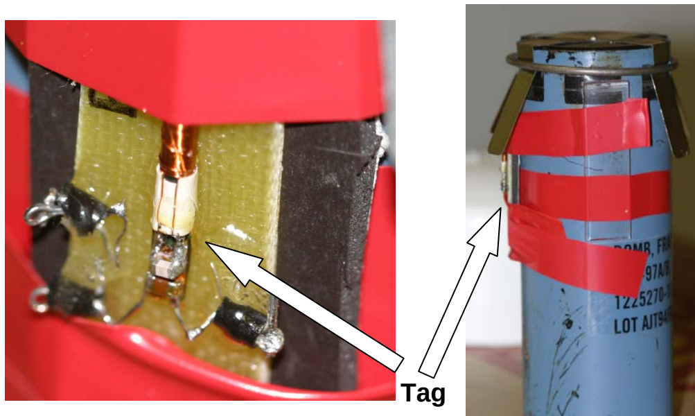
Figure 36. Tiris solenoidal tag mounted on a BLU-97
