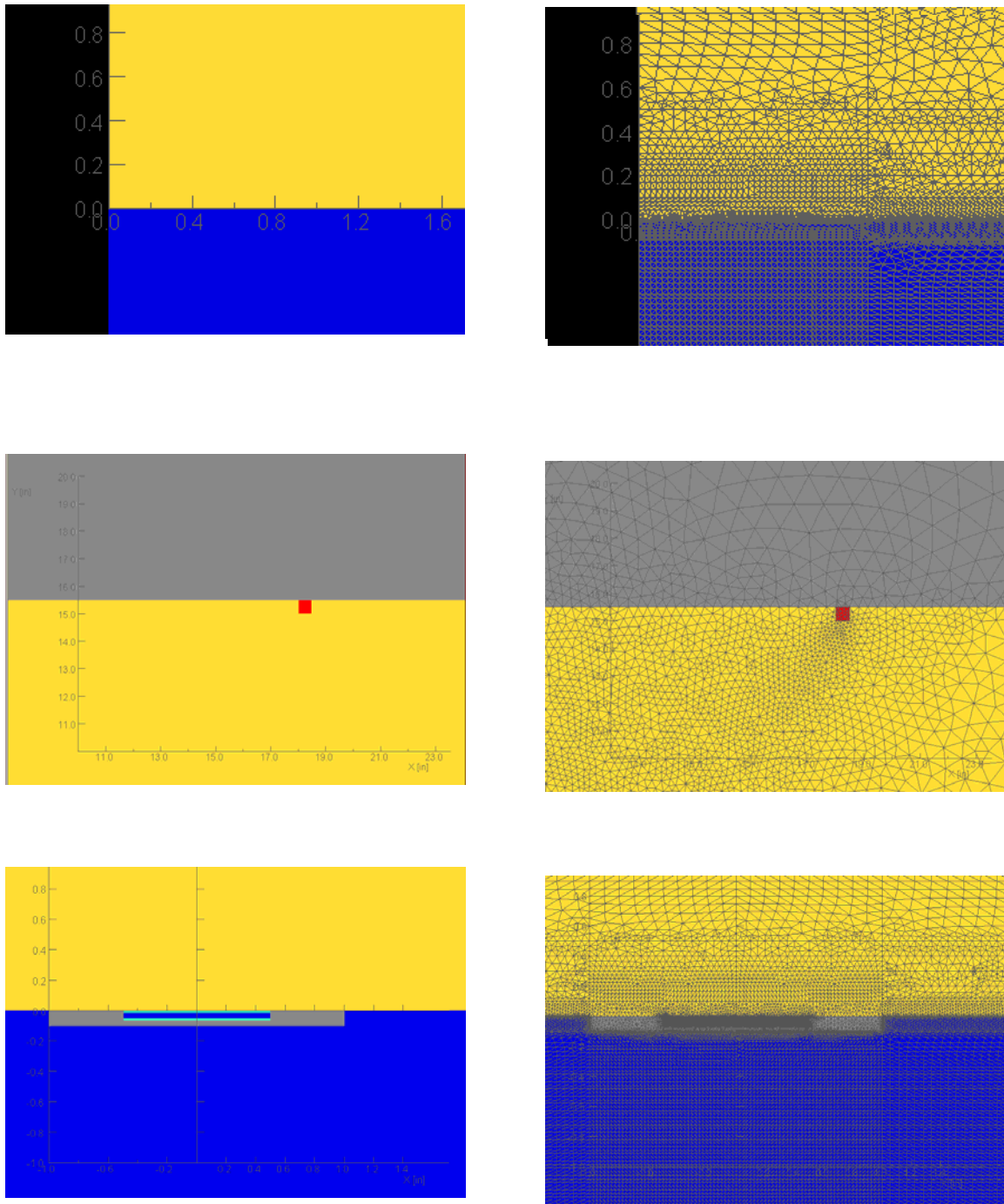
Figure 91. Examples of Mesh near the munition surface (top), the transmitting coil (center), and the munition groove and EM tag (bottom). These meshes yielded errors less than two percent in the regions of interest.
