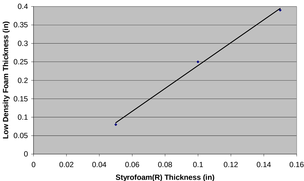
Figure 67. Equivalent thickness of Styrofoam® for a given thickness of low-density foam
