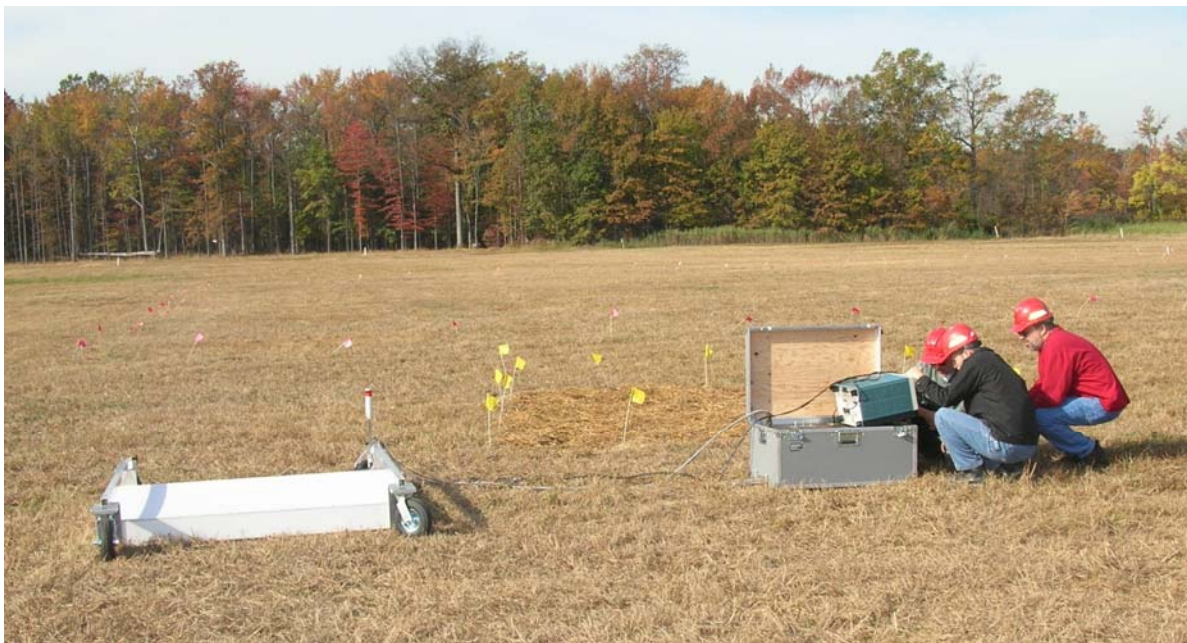
Figure 72. Coil module and electronics module being used at Aberdeen Test Center in 2005
