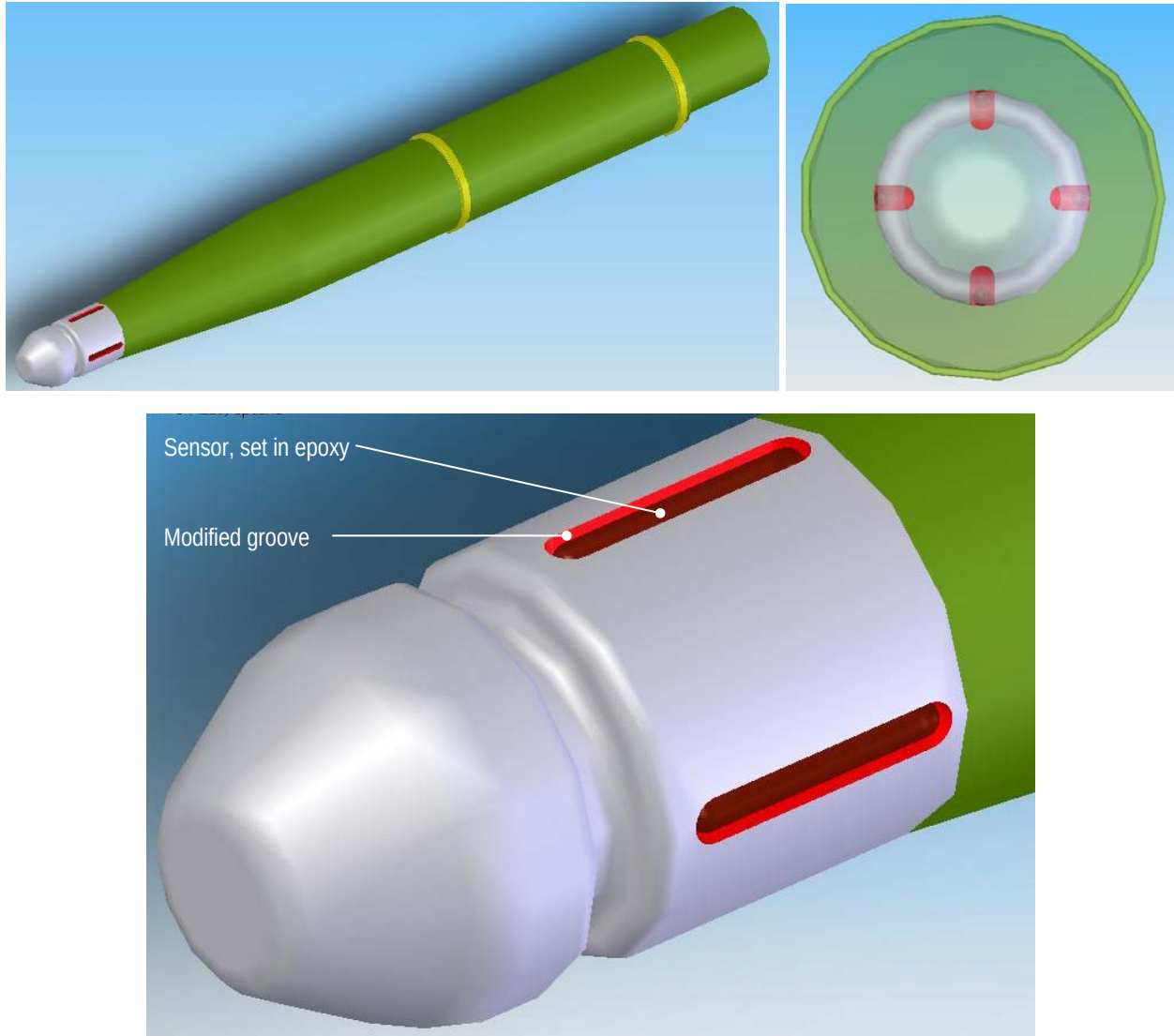
Figure 22. M229 mounting option
