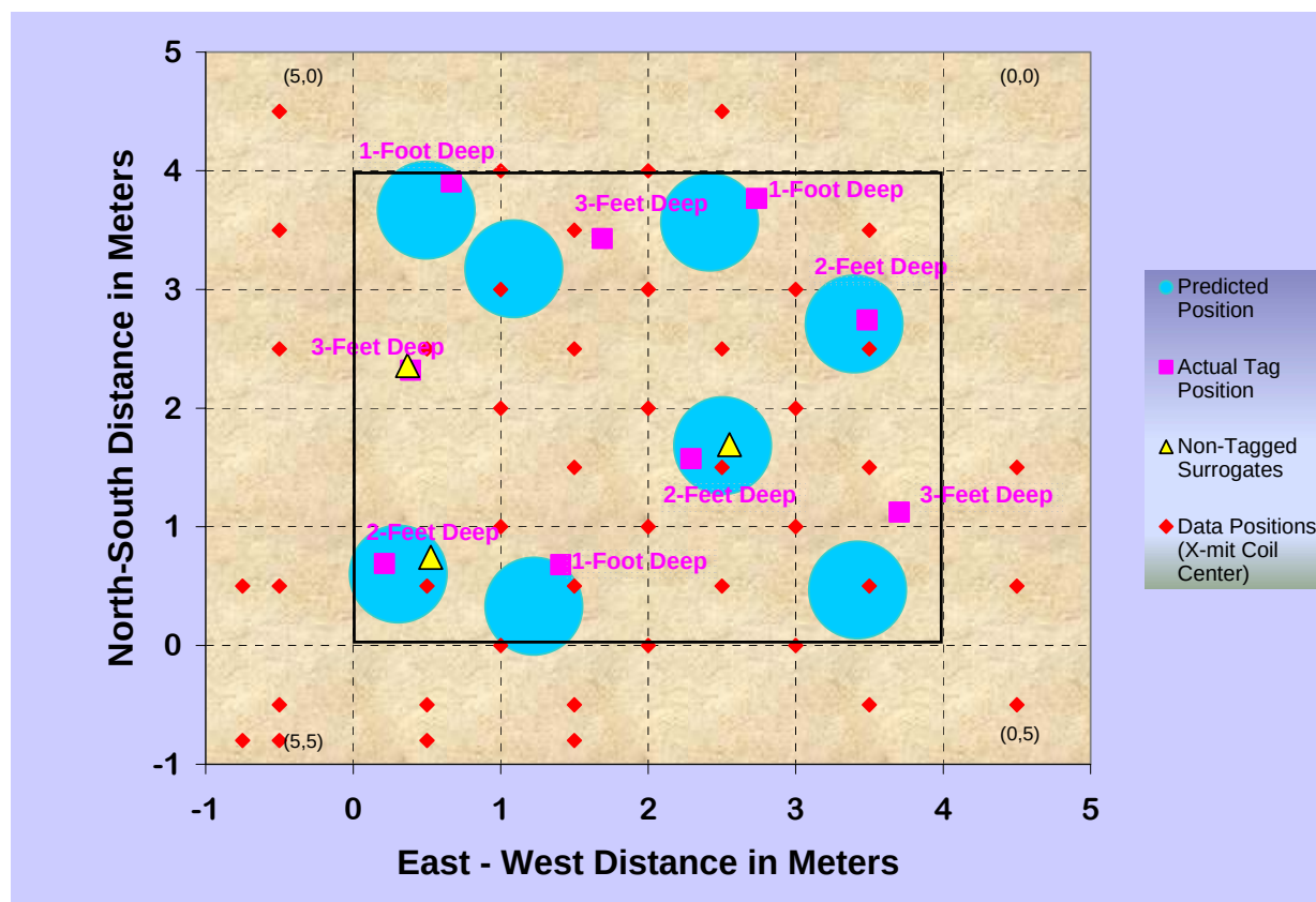
Figure 74. Plan view of the 2005 test grid at Aberdeen Test Center showing the actual tagged munition positions, Battelle's predicted positions, and the positions where Battelle acquired data
