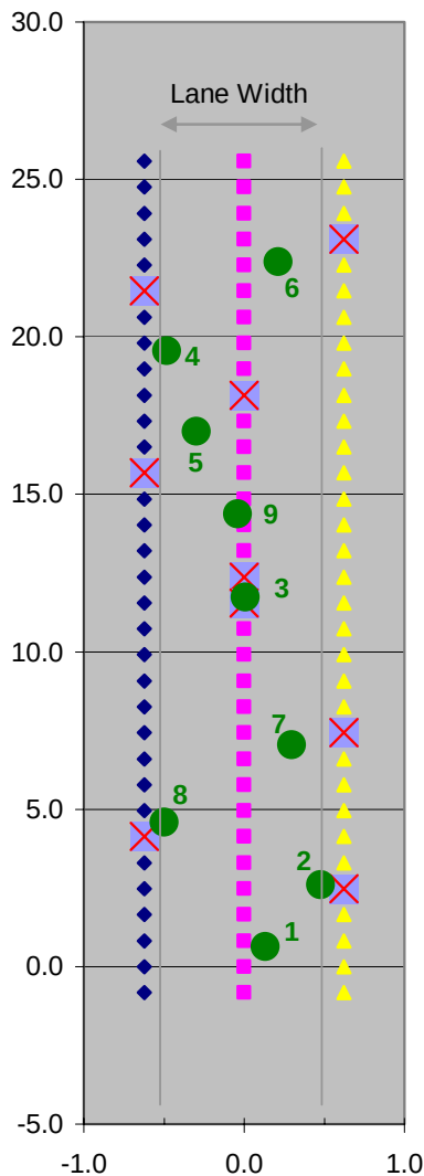
Figure 78. Plan view of the tagged ordnance items buried at Aberdeen Test Center in 2006. The test lane was one meter wide and 25 meters long; the lane width and length scales in the figure are not identical. The blue diamonds, magenta squares, and yellow triangles represent data acquisition locations. The blue squares with red crosses indicate Battelle's estimate of surrogate locations and the numbered round green circles indicate the actual surrogate positions.
