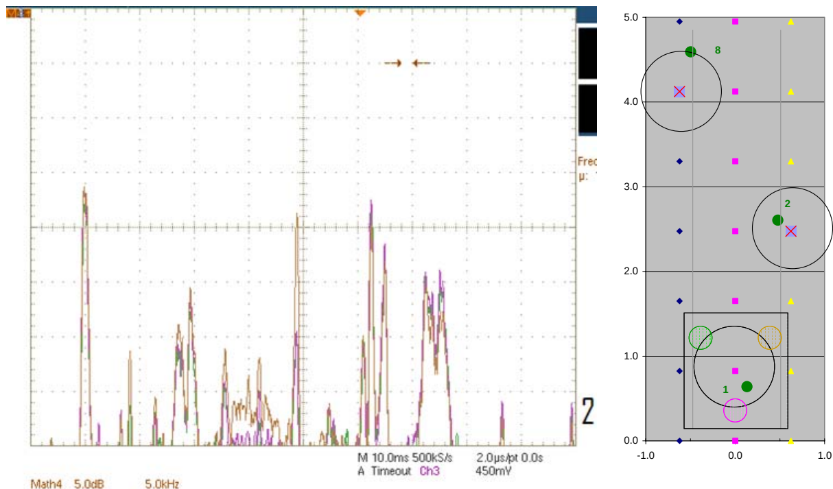
Figure 83. The plot shows data taken at point (2, C), which was directly over surrogate 1. The relevant portion of the test lane is shown on the right, with the position of the interrogation module, including its transmit coil and three receive coils
