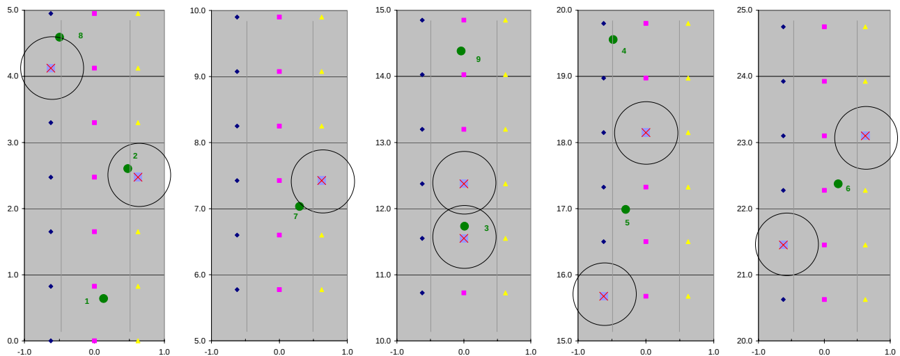
Figure 80. Plan view of the 2006 test lane divided into five equal segments. The data acquisition positions are shown as blue diamonds, red squares, or yellow triangles. ATC emplacements are shown as numbered green circles and Battelle's estimates are shown with red X symbols inside 1-m diameter circles that symbolize the size of the resolution area of Battelle's estimates
