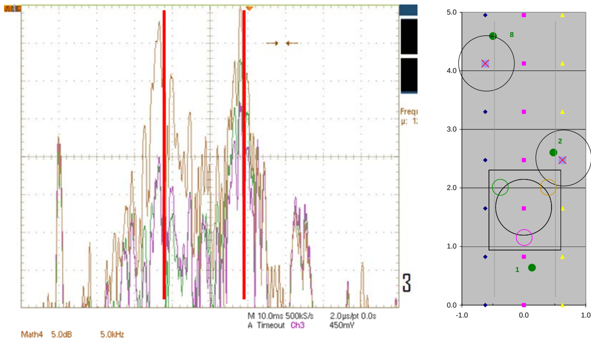
Figure 82. Example data plot with coil module positioned above a tagged surrogate. The signal strength is much higher at the two cursor positions indicated by the vertical red lines. The signal is strongest in the brown receive coil, which is near surrogate 2
