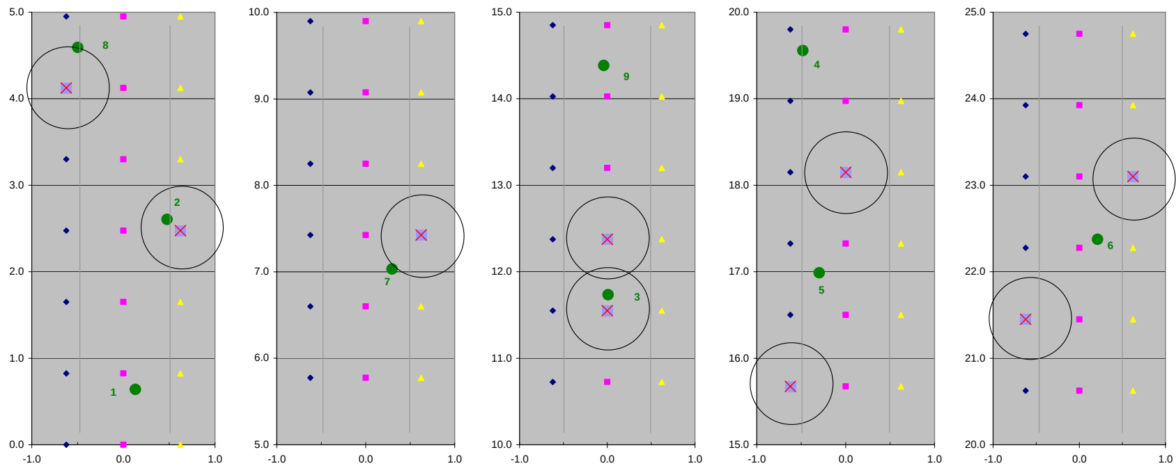
Figure 95. Plan view of the grid at ATC. The data acquisition positions are shown as blue diamonds, red squares, or yellow triangles. ATC emplacements are shown as numbered green circles and Battelle's estimates are shown with red X symbols inside 1-m diameter circles that symbolize the size of the resolution area of Battelle's estimates.
