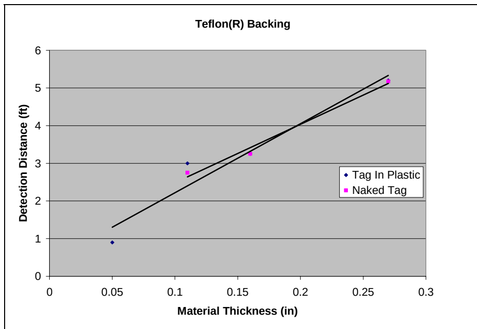
Figure 62. Detection distance as a function of Teflon backing thickness when Trolley Scan RF tag is placed on a conductor
