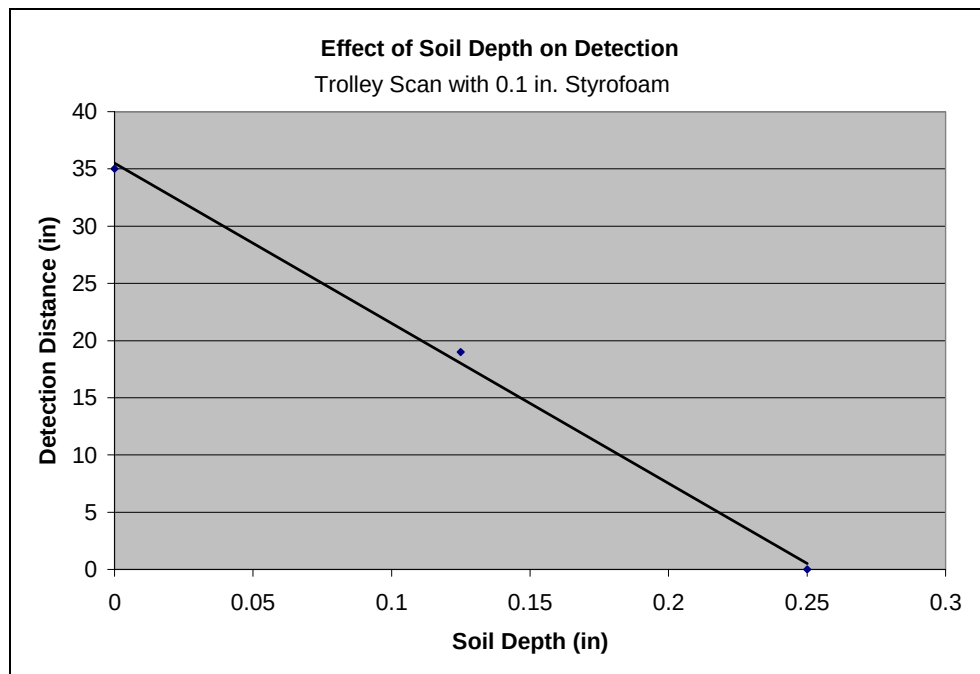
Figure 51. Effect of soil depth on detection distance for the Trolley Scan RF tag
