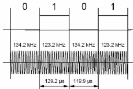
Figure 34. Details of the tag's reply signal showing the timing of the two FSK frequencies
