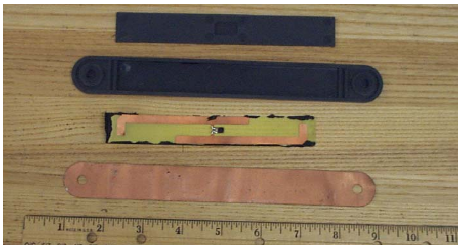
Figure 64. Disassembled APT-1014 AWID tag
