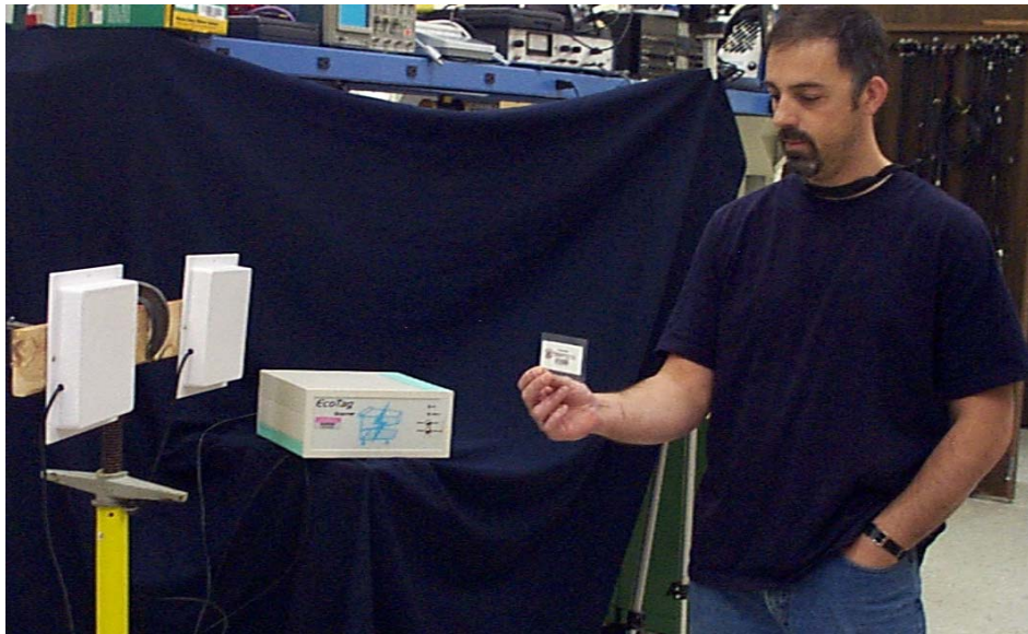
Figure 46. Laboratory setup of range and azimuth measurements with the Trolley Scan RF tag system
