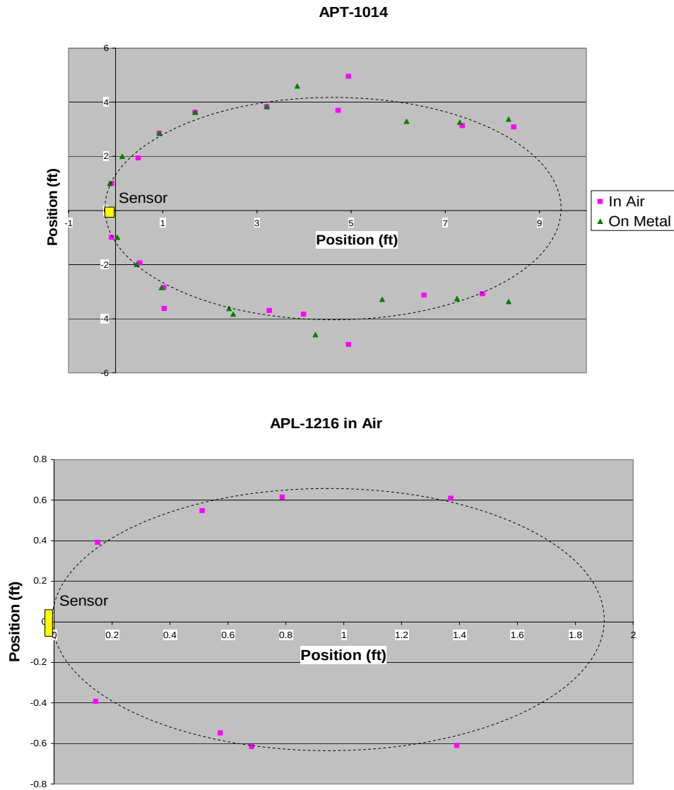
Figure 39. Laboratory measurements of AWID UHF tag range versus azimuth angle
