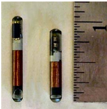
Figure 1. The Tiris RFID tags selected to aid detection of buried UXO
