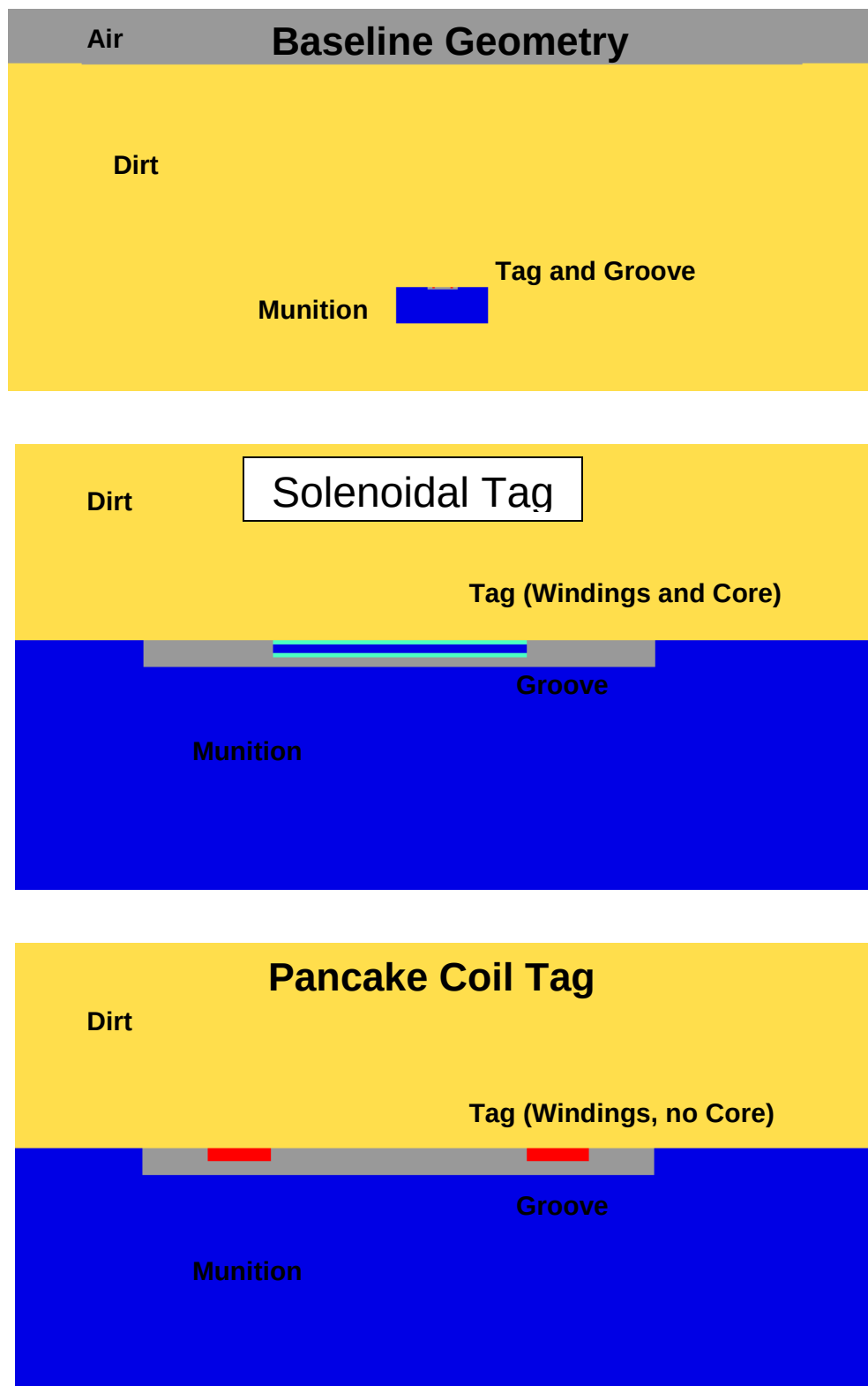
Figure 90. Geometry Examples for the case of transmitting a signal from the EM tag. Both Types of EM tags are shown
