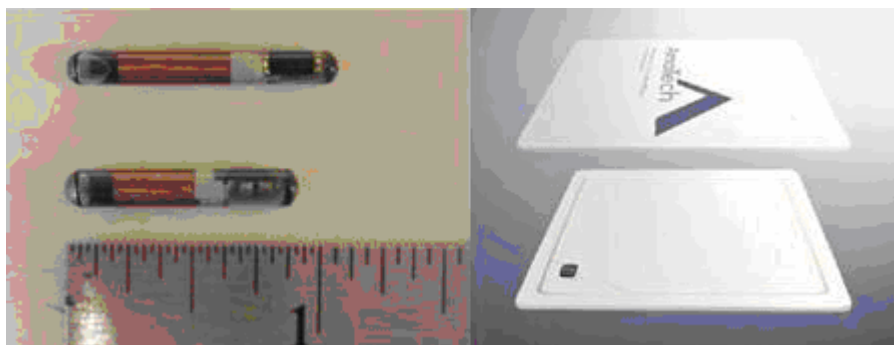
Figure 92. Solenoidal tags on the left and "pancake" tags on the right
