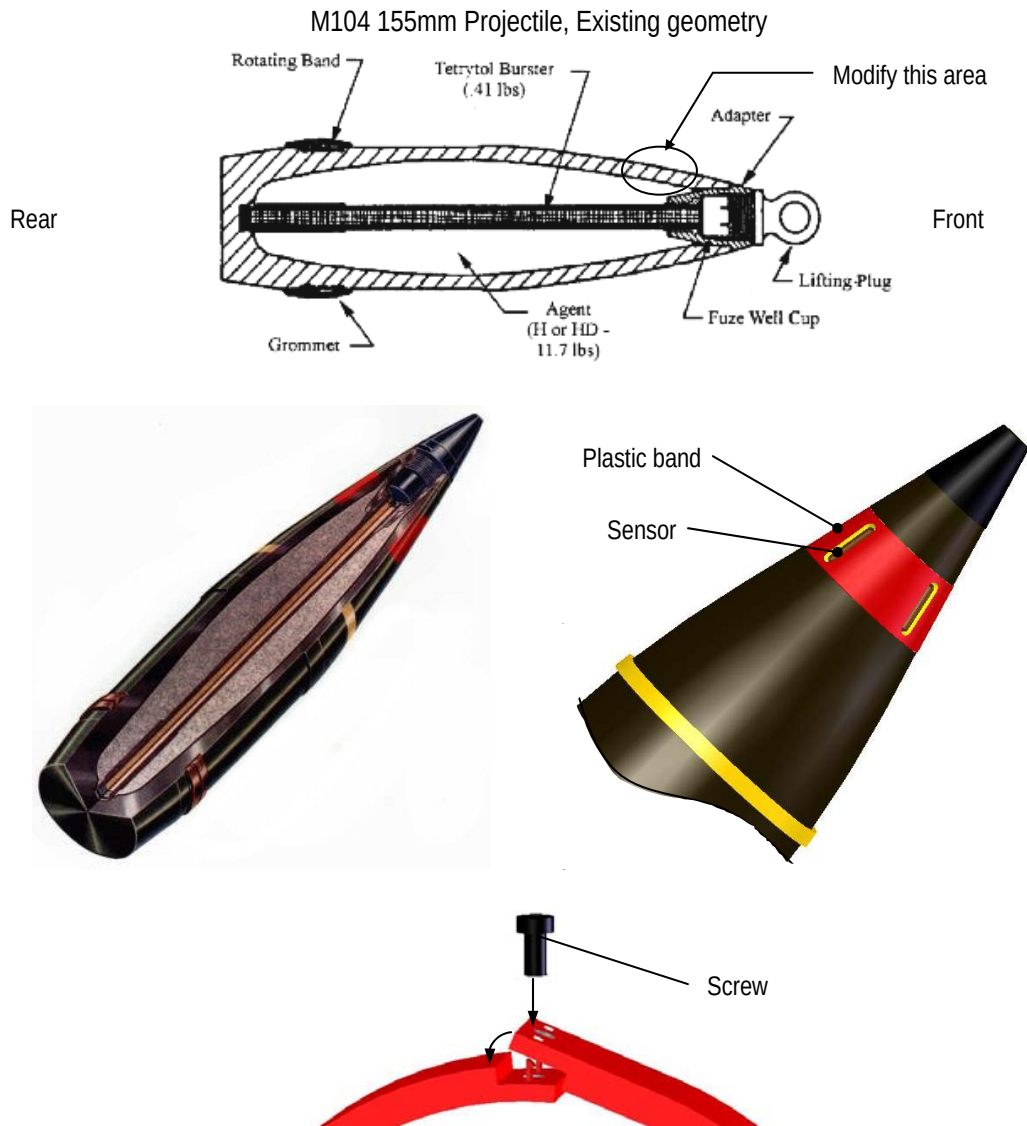
Figure 24. 155mm projectile, M1XX bursting: tagging recommendation
