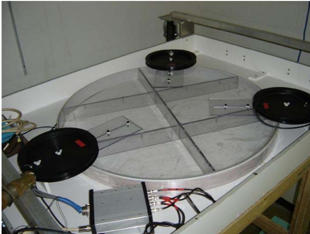
Figure 71. The interior of the coil module showing the one-meter diameter transmit coil and the three separate receive coils
