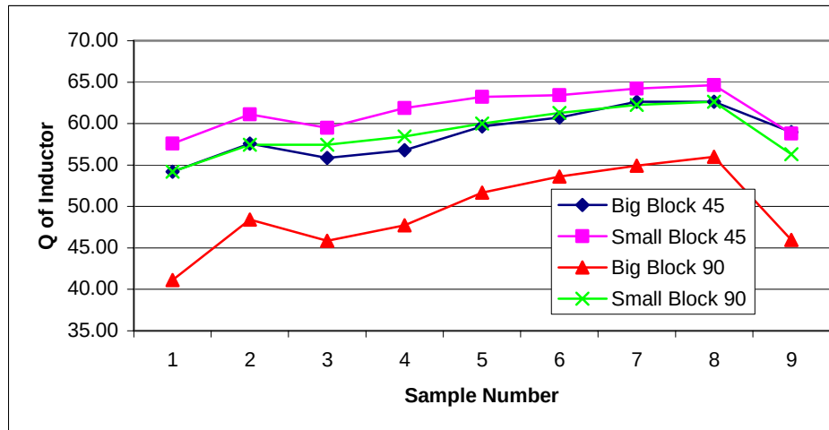
Figure 87. Sample result of varying block size and wall angle. The sample number refers to lengths and widths of the void around the steel walls
