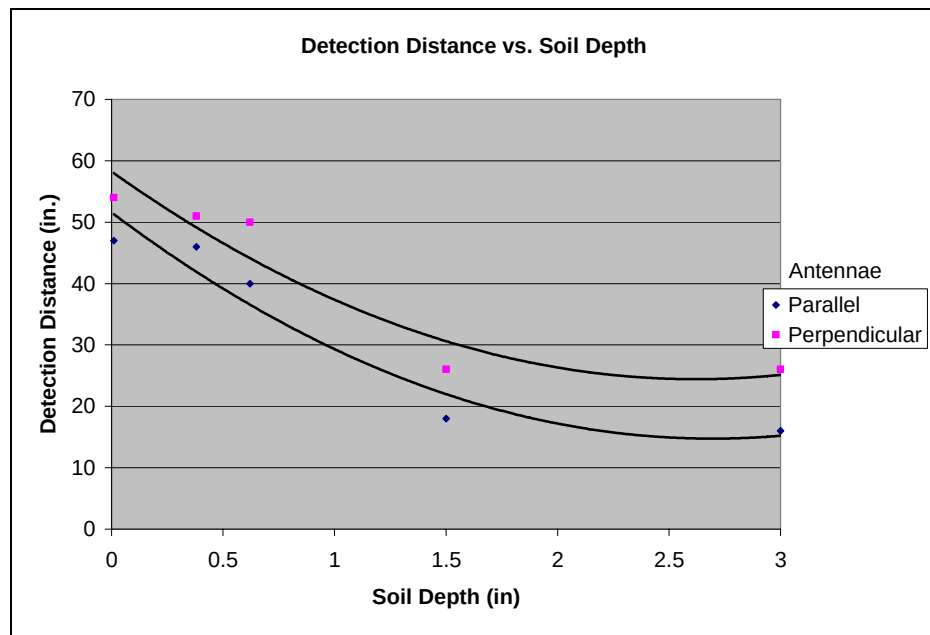
Figure 58. Matrics tag detection range as a function of soil depth
