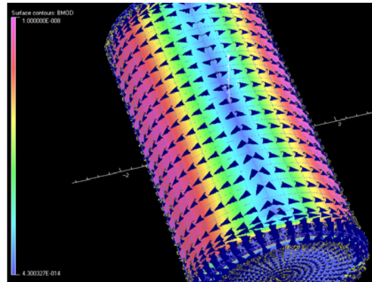
Figure 3. Depiction of the theoretical magnetic field levels near the surface of a cylindrically-shaped munition surrogate
