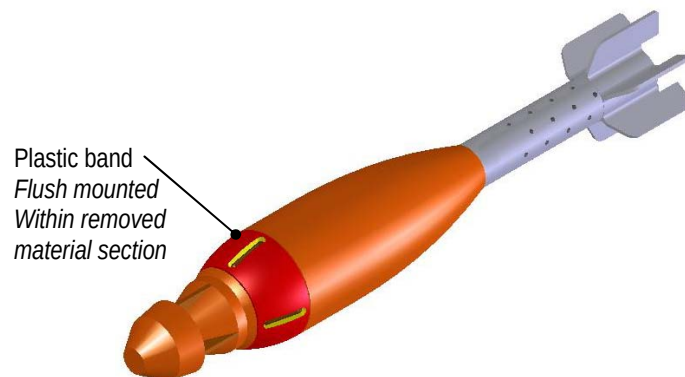
Figure 16. 60mm cartridge Option 2
