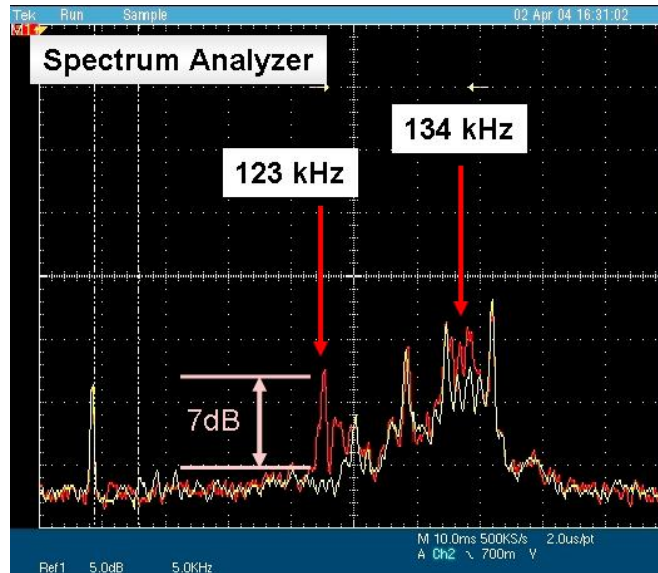
Figure 33. Spectrum analyzer view of the Tiris tags that use frequency shift keying between about 123 kHz and 134 kHz. This data set was obtained with 32-mm solenoidal tag 0.29 inches from BLU-97 surface with the tag response averaged over 50 samples.
