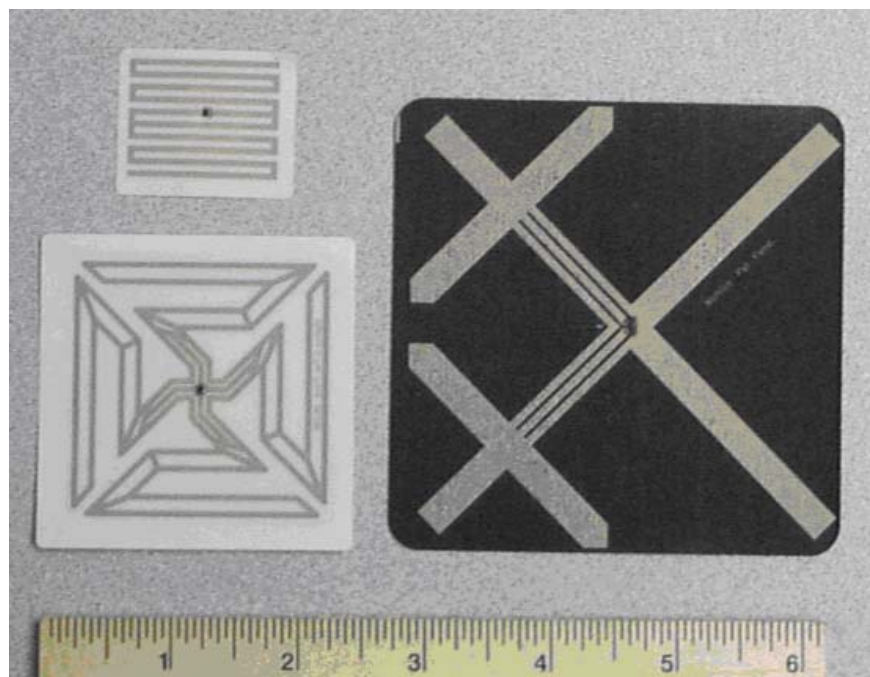
Figure 52. Matrics AR-400 tag configurations
