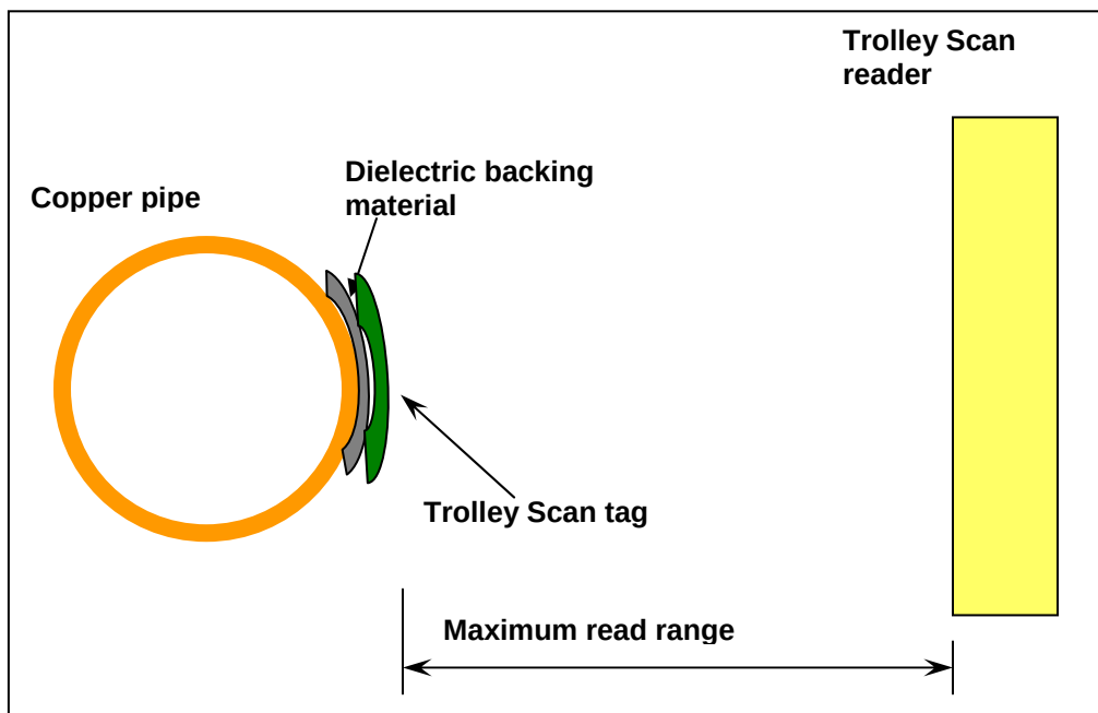
Figure 60. Measurement geometry for tests with backing materials
