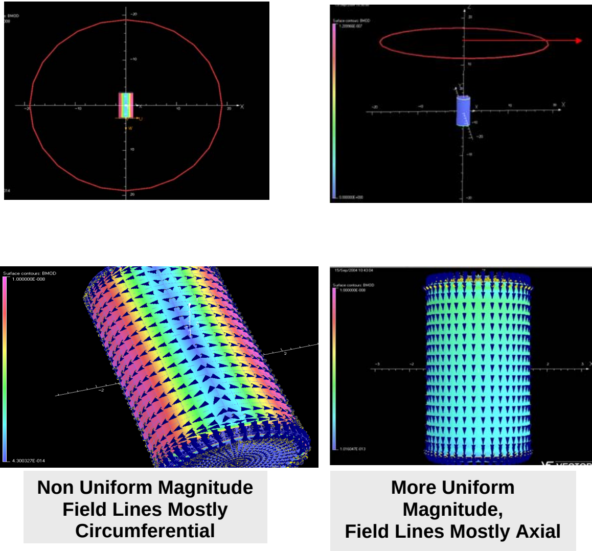
Figure 27. This figure shows the finite element analysis outputs. Both examples show the magnetic field intensity and vector direction for the interrogating coil directly above a horizontally-oriented (left) and a vertically-oriented (right) munition. The units are Tesla per Amp-Turn and the range of colors is between 4.3 \times 10^{-14} (blue) and 1 \times 10^{-8} (magenta)
