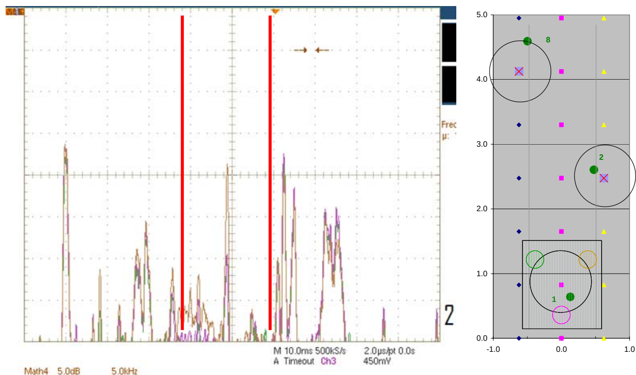
Figure 81. Example data plot with no tagged surrogate present. The plot provides frequency as the horizontal axis and signal strength in dB along the vertical axis. The drawing on the right shows the position of the interrogation module in the test lane when the data was acquired.
