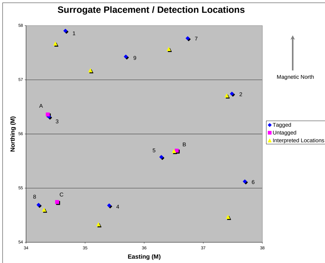
Figure 77. Aberdeen Test Center's plot of the 2005 data shown in Figure 74
