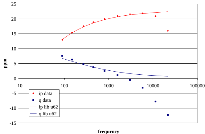
Figure 17. An example of high-frequency underwater spectral distortion resulting in a UXO classified as clutter. This example, at 20 cm lateral offset and 45 cm height, was from the aluminum pipe; non-ferrous ordnance systematically gives larger misfits even though EMIS gives the correct identification.
