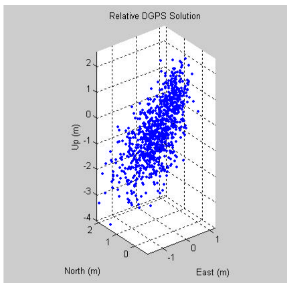
Figure 16 HAGR DGPS Position Solution
