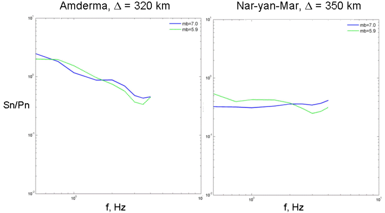
Figure 28. Comparison of Sn/Pn spectral ratios for Southern Novaya Zemlya explosions of 9/27/73 ( m_b = 5.9 ) and 10/27/73 ( m_b = 7.0 ) at stations Amderma (left) and Nar-yan-Mar (right).
