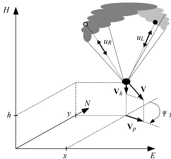
Figure 1: System SKY MULE – basic parameters (control cords are denoted by dotted lines with arrows u_L, u_R representing “left” and “right” control signals).
