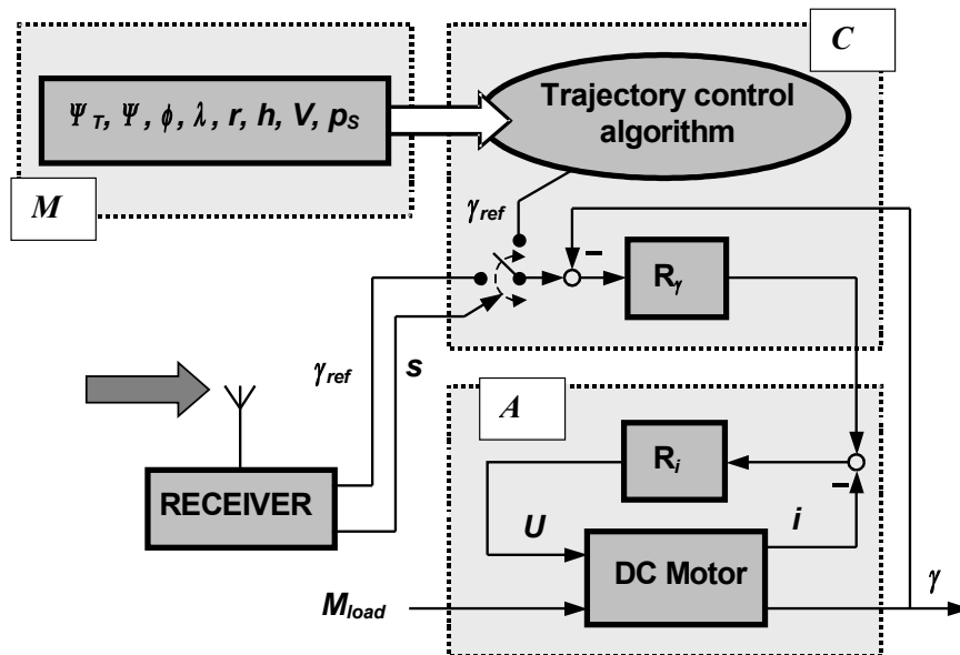
Figure 2: Simplified structure of the control module.
