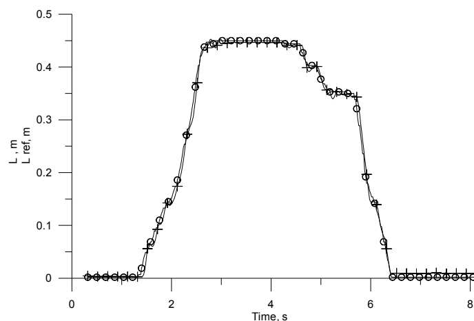
Figure 4: The result of manual excitation of the actuator. “Crosses” marked curve - the actual position of actuator's rack belt ( L ), “circles” marked curve – manually generated signal representing the desired position of this rack belt ( L_{ref} ).
