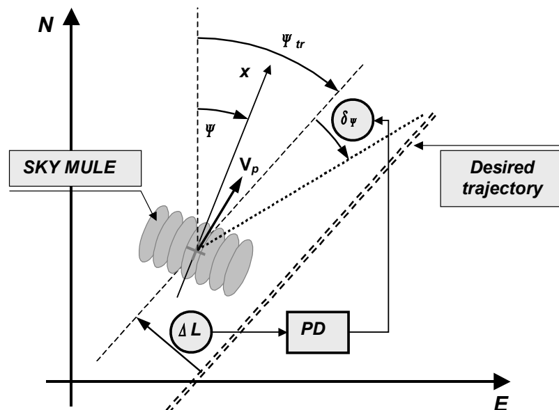
Figure 8: Trajectory control – definition of correcting term \delta_{\psi} for desired heading \Psi_{ref} .
