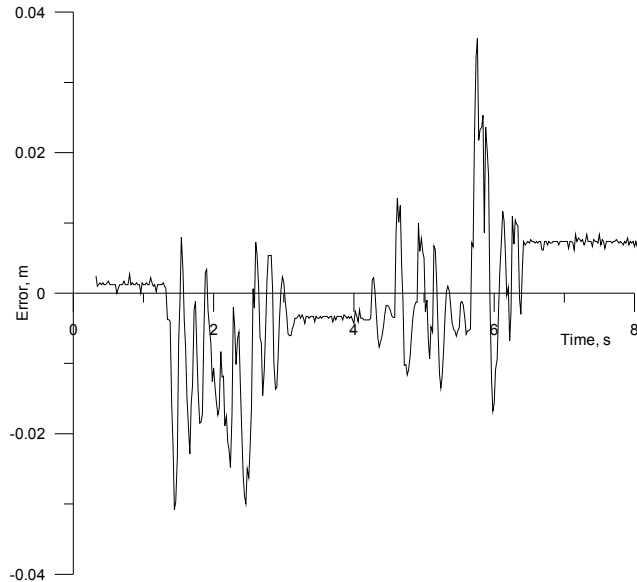
Figure 5: Control error for the result depicted on Figure 4 – the difference L - L_{ref} .
