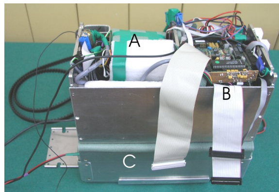
Figure 6: The control module with removed lid of the housing and control computer (section B) taken out. Measuring unit is installed in section A and actuators with batteries in section C.
