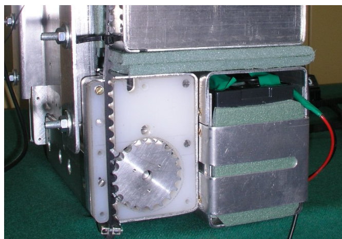
Figure 3: Actuator's gear - rack wheel and rack belt are visible after removing gear's lid.
